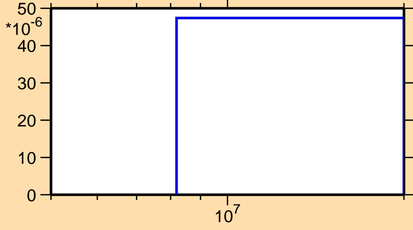
\sigma vs. E for ^{172}\text{Os}(n,t)
