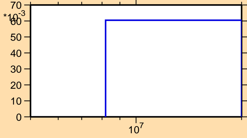
\sigma vs. E for ^{172}\text{Os}(n,2n)
