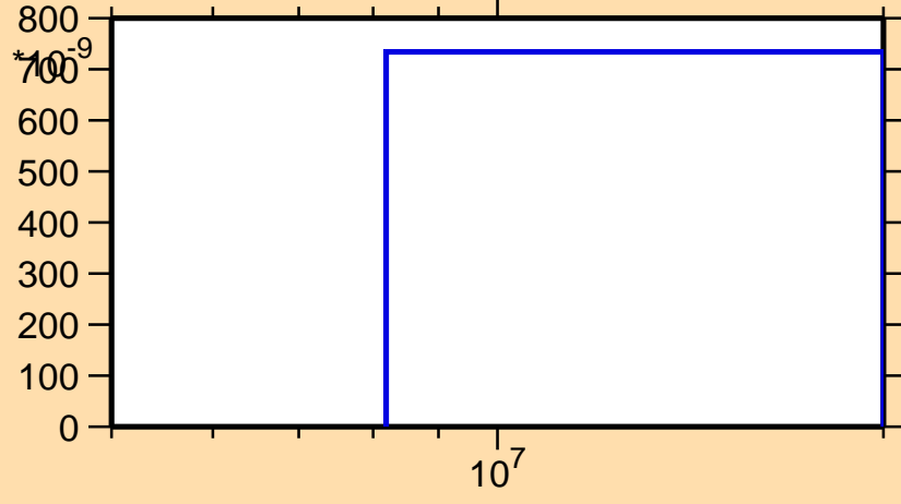
\sigma vs. E for ^{172}\text{Os}(n,\text{pd})
