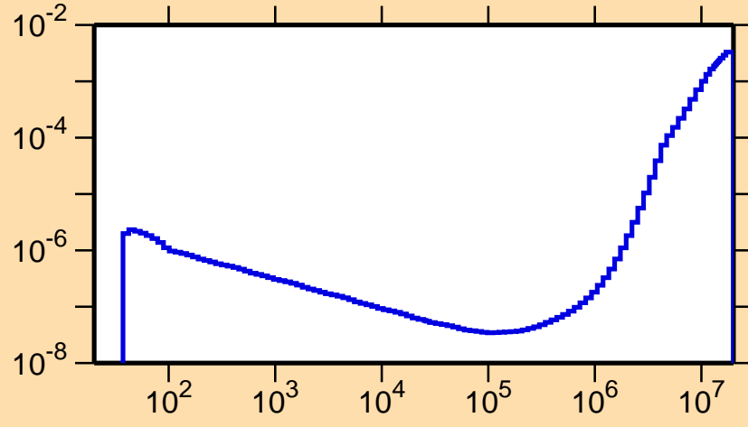
\sigma vs. E for ^{173}\text{Os}(n,p\alpha)
