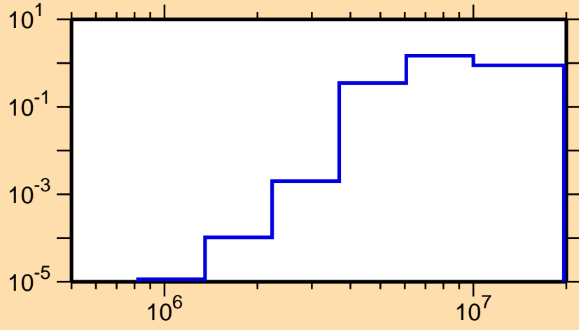
\sigma vs. E for ^{173}\text{Os}(n,n\text{cont.})
