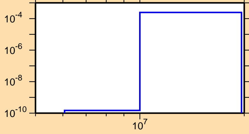
\sigma vs. E for ^{173}\text{Os}(n,t)
