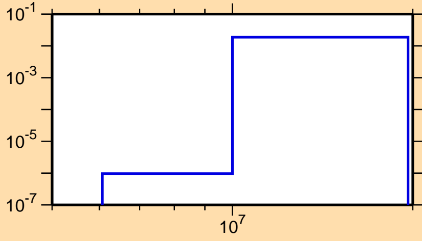
\sigma vs. E for ^{173}\text{Os}(n,2n\alpha)
