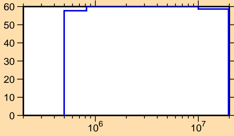
\Delta\sigma/\sigma vs. E for ^{173}\text{Os}(n,n\text{cont.})
