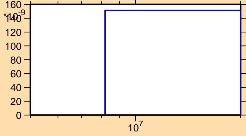
\sigma vs. E for ^{173}\text{Os}(n,\text{nd})
