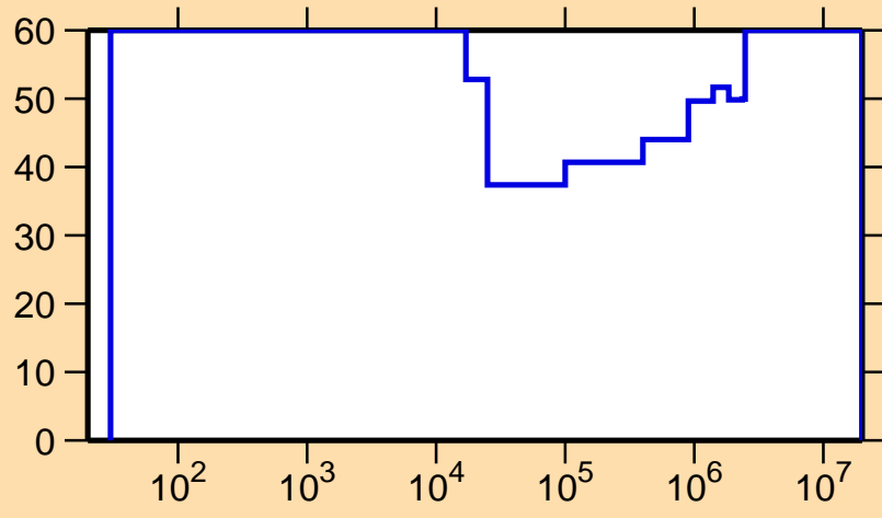
\Delta\sigma/\sigma vs. E for ^{173}\text{Os}(n,\gamma)
