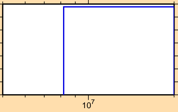
\sigma vs. E for ^{173}\text{Os}(n,nt)
