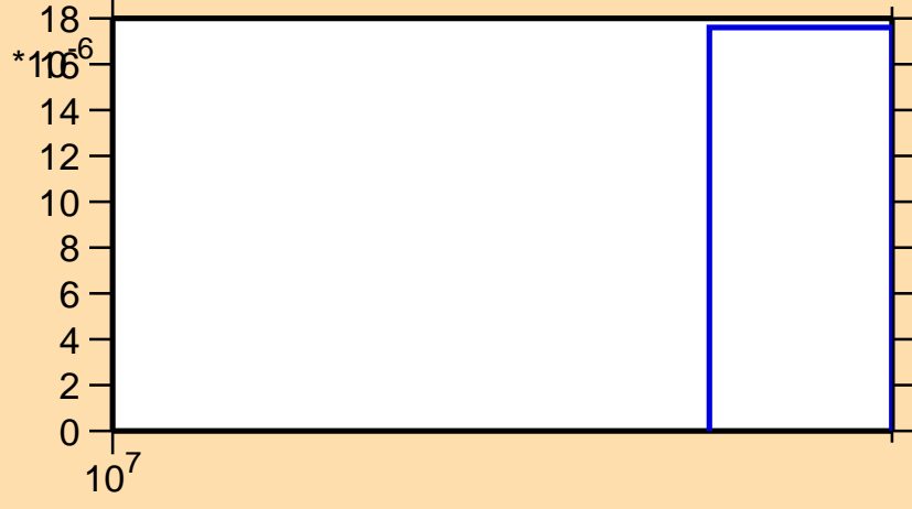
\sigma vs. E for ^{174}\text{Os}(n,3n)
