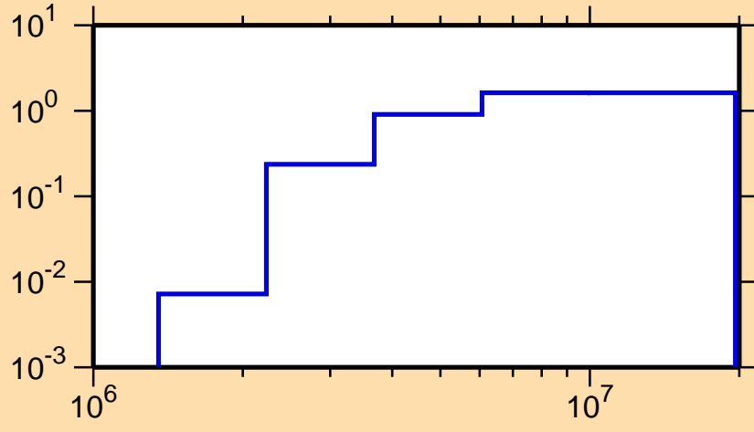
\sigma vs. E for ^{174}\text{Os}(n,n\text{cont.})
