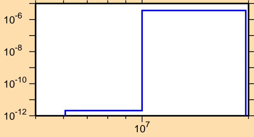
\sigma vs. E for ^{174}\text{Os} (mt 45)
