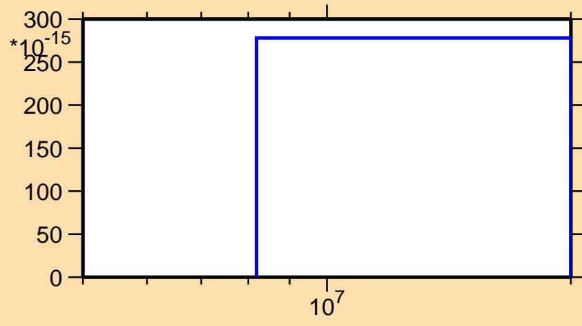
\sigma vs. E for ^{174}\text{Os} (mt 34)
