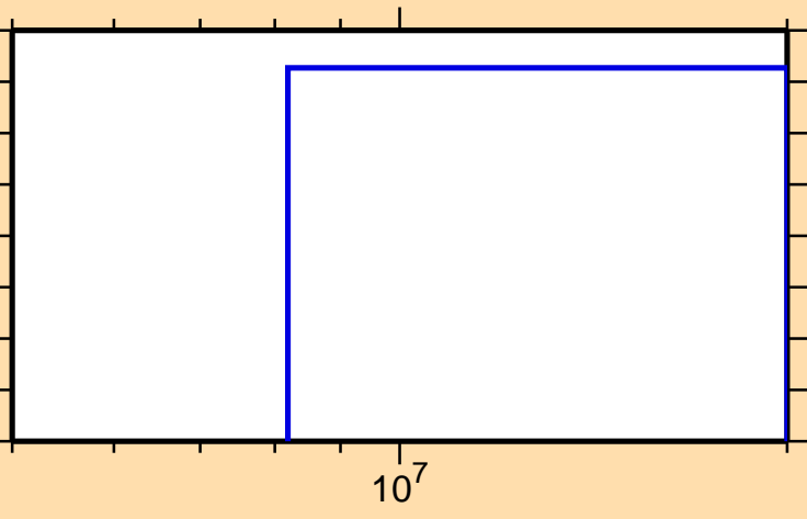
\sigma vs. E for ^{174}\text{Os}(n,2np)
