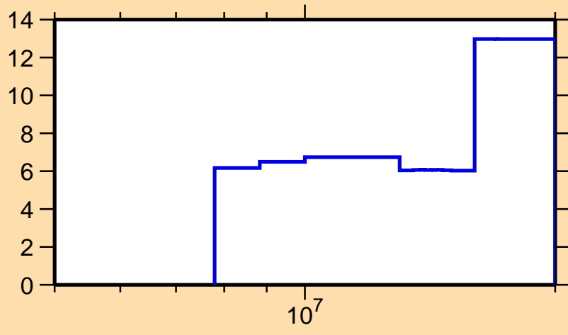
\Delta\sigma/\sigma vs. E for ^{175}\text{Os}(n,\text{tot.})
