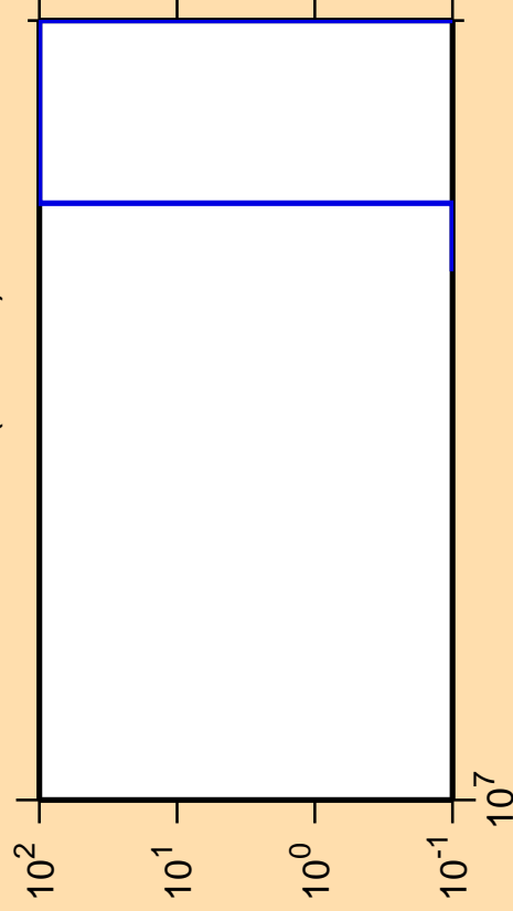
\Delta\sigma/\sigma vs. E for ^{175}\text{Os}(n,3n\alpha)
