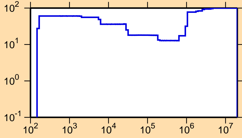
\Delta\sigma/\sigma vs. E for ^{175}\text{Os}(n,\gamma)
