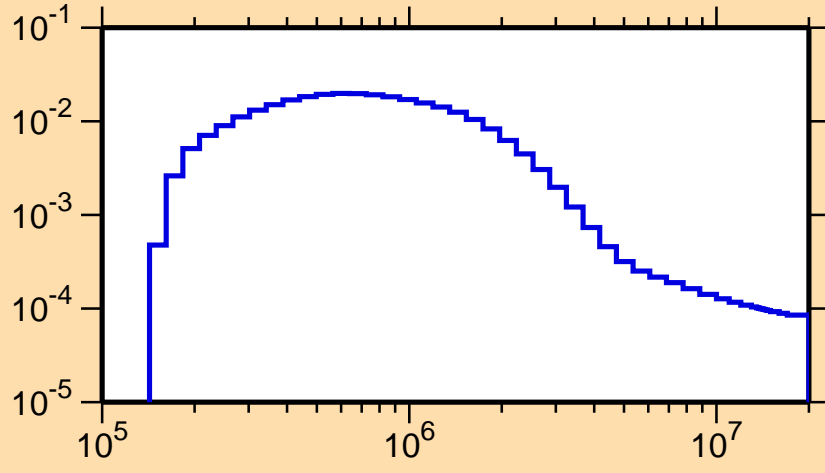
\sigma vs. E for ^{175}\text{Os}(n,n_4)
