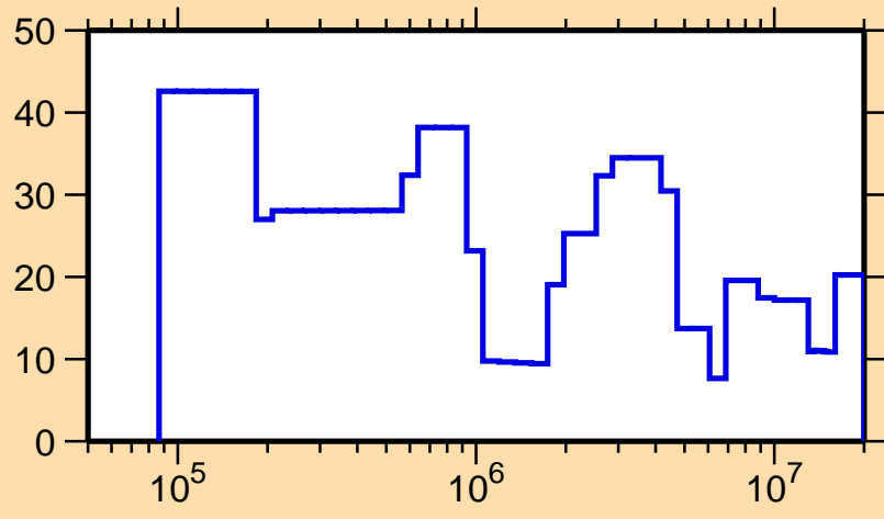
\Delta\sigma/\sigma vs. E for ^{175}\text{Os}(n,\text{el.})
