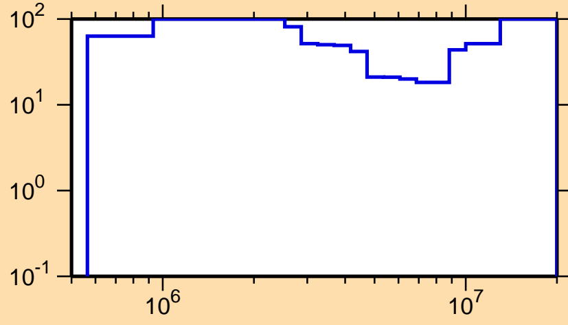
\Delta\sigma/\sigma vs. E for ^{175}\text{Os}(n,n\text{cont.})
