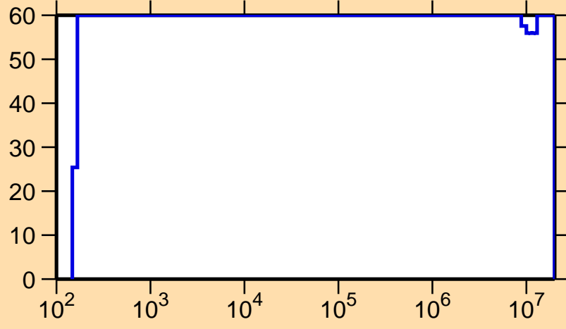
\Delta\sigma/\sigma vs. E for ^{175}\text{Os}(n,p)
