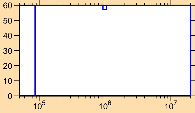
\Delta\sigma/\sigma vs. E for ^{175}\text{Os}(n,n_1)
