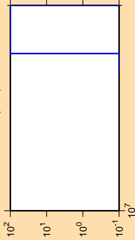
\Delta\sigma/\sigma vs. E for ^{175}\text{Os}(n,nt)
