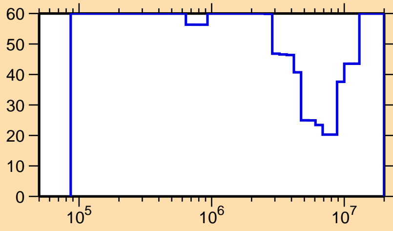
\Delta\sigma/\sigma vs. E for ^{175}\text{Os}(n,\text{inel.})
