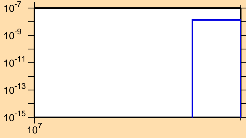
\sigma vs. E for ^{175}\text{Os}(n,3n\alpha)
