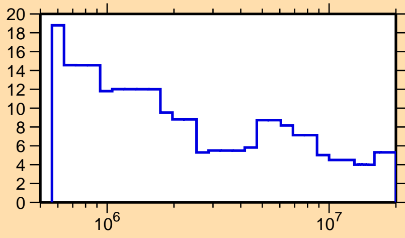
\Delta\sigma/\sigma vs. E for ^{175}\text{Os}(n,\text{nonel.})
