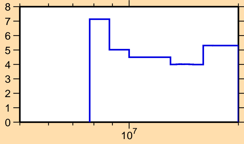
\Delta\sigma/\sigma vs. E for ^{175}\text{Os}(n,\text{nonel.})
