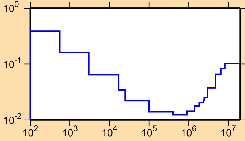
\sigma vs. E for ^{175}\text{Os}(n,p)
