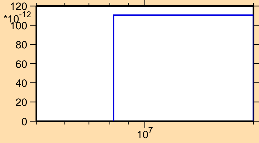
\sigma vs. E for ^{175}\text{Os}(n,3n\alpha)
