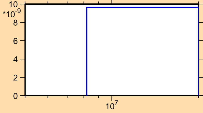
\sigma vs. E for ^{175}\text{Os}(n,\text{pd})
