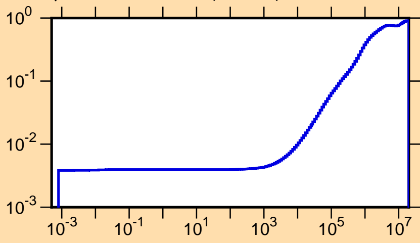
\mu vs. E for ^{176}\text{Os}(\text{mt251})
