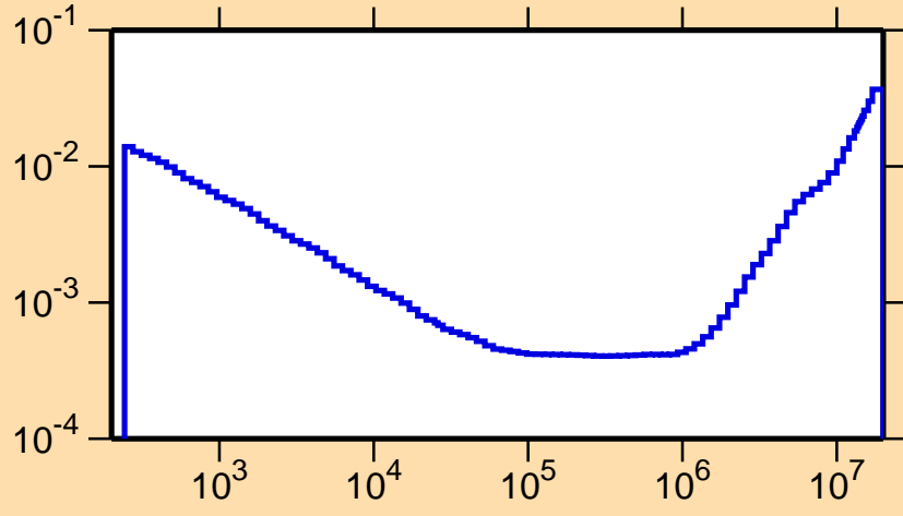
\sigma vs. E for ^{176}\text{Os}(n,\alpha)
