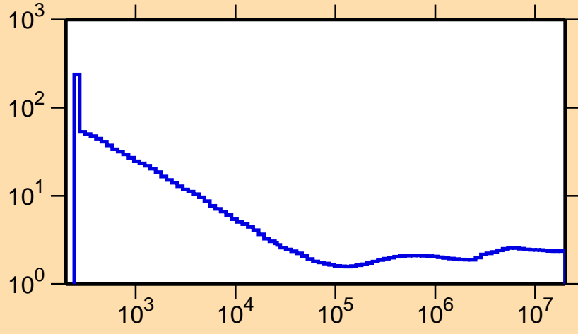
\sigma vs. E for ^{176}\text{Os}(n,\text{nonel.})
