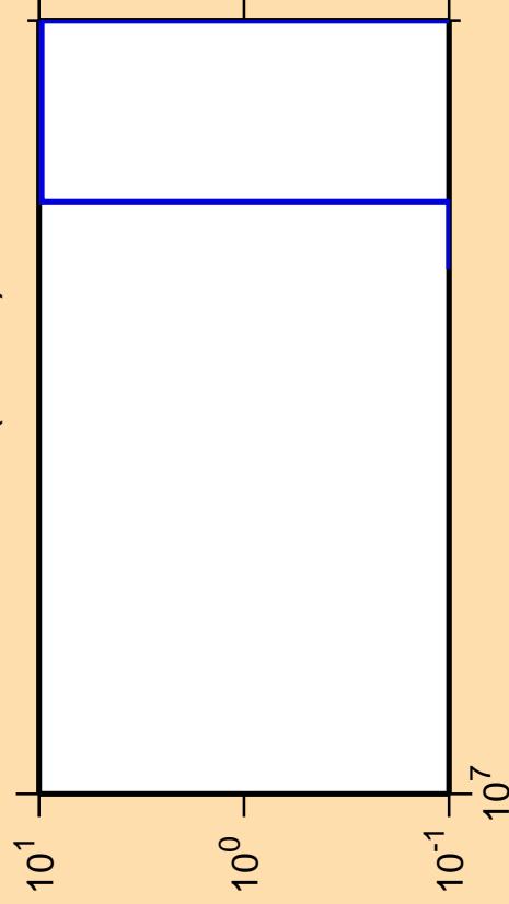
\Delta\sigma/\sigma vs. E for ^{177}\text{Os}(n,3n\alpha)
