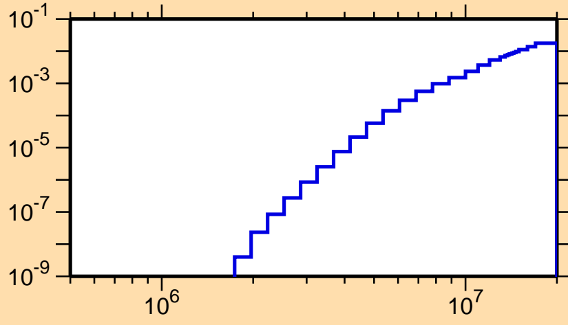
\sigma vs. E for ^{177}\text{Os}(n,n\alpha)
