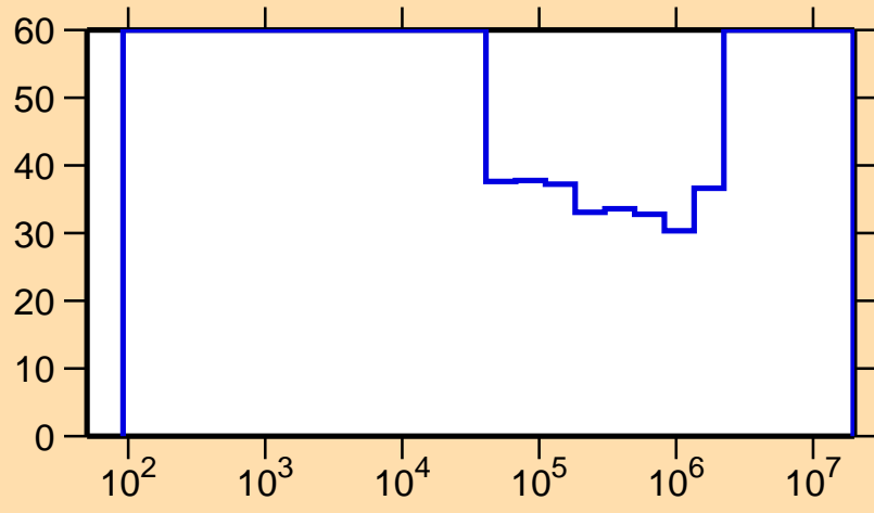
\Delta\sigma/\sigma vs. E for ^{177}\text{Os}(n,\gamma)
