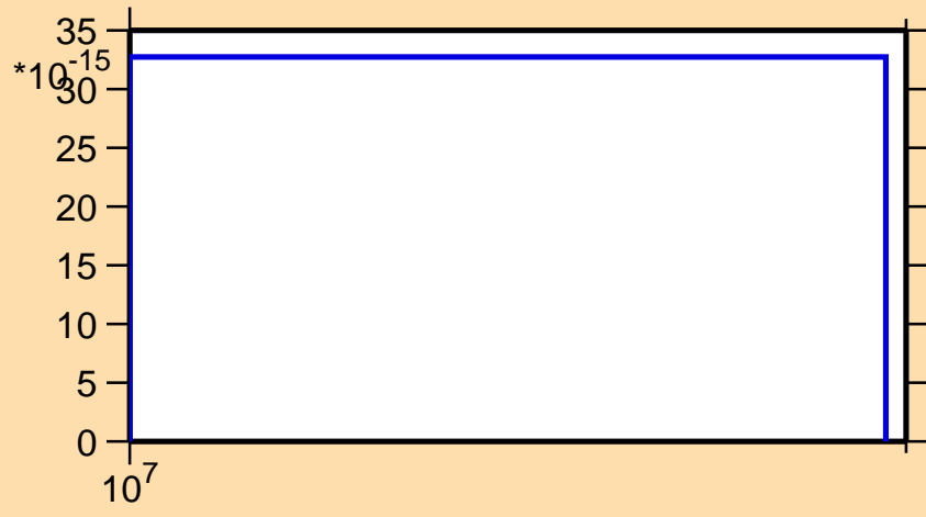
\sigma vs. E for ^{177}\text{Os}(n,3n\alpha)
