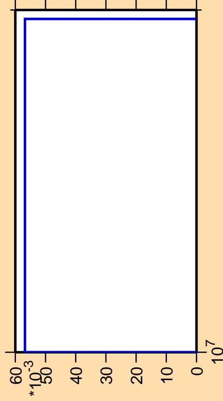
\Delta\sigma/\sigma vs. E for ^{177}\text{Os}(n,3n\alpha)
