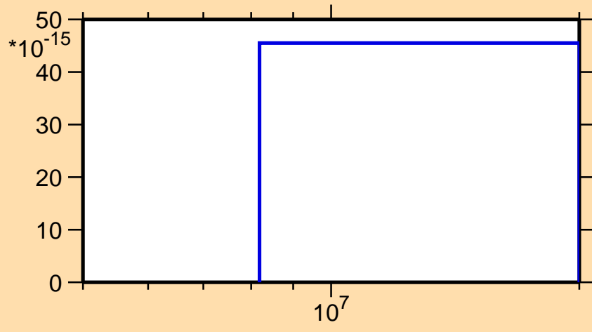
\sigma vs. E for ^{177}\text{Os}(n,3n\alpha)
