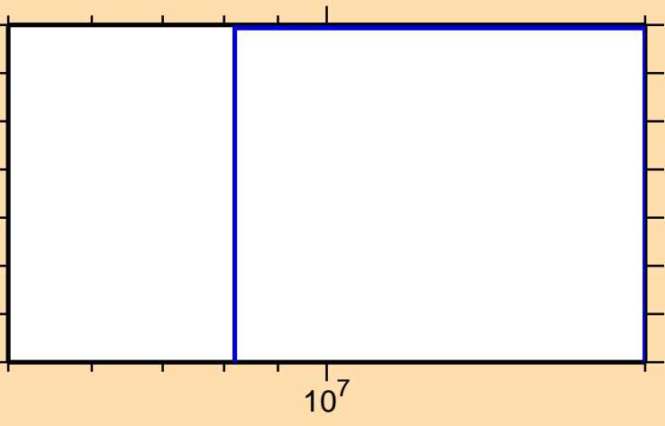
\sigma vs. E for ^{177}\text{Os}(n,\text{nd})
