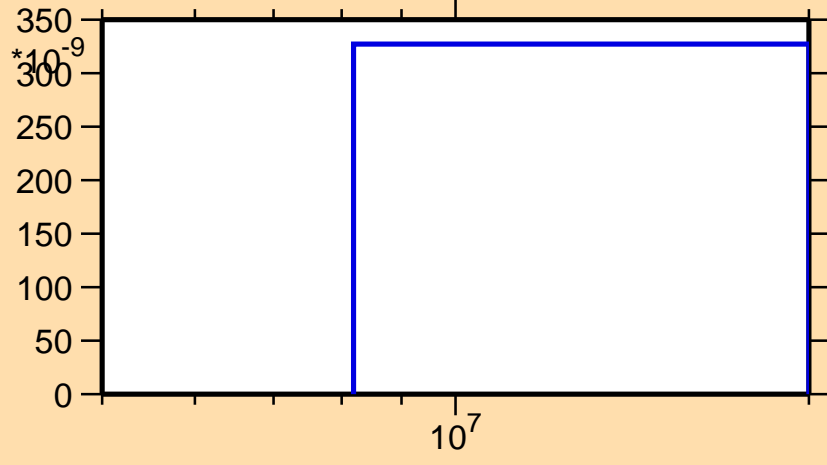
\sigma vs. E for ^{177}\text{Os}(n,\text{He}3)
