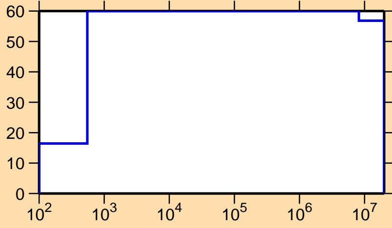
\Delta\sigma/\sigma vs. E for ^{178}\text{Os}(n,p)
