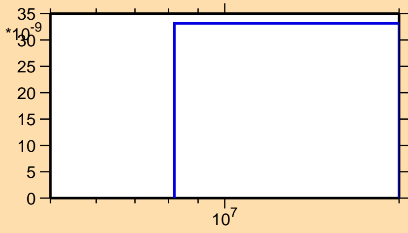
\sigma vs. E for ^{178}\text{Os}(n,\text{He}3)
