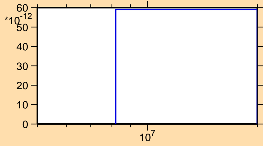
\sigma vs. E for ^{178}\text{Os}(n,3n\alpha)
