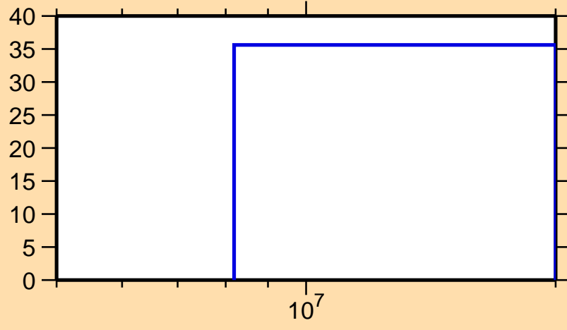
\Delta\sigma/\sigma vs. E for ^{178}\text{Os}(n,2n)
