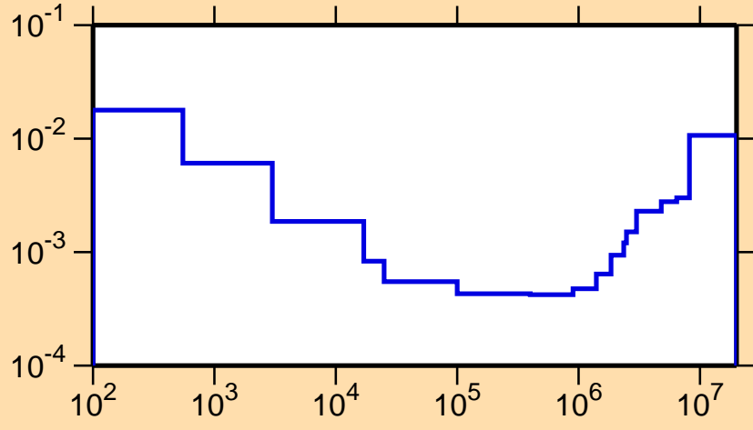
\sigma vs. E for ^{178}\text{Os}(n,\alpha)
