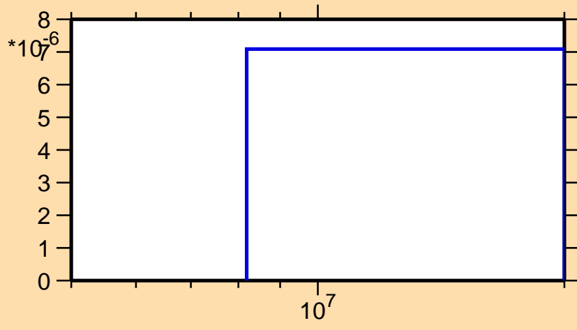
\sigma vs. E for ^{178}\text{Os}(n,2n\alpha)
