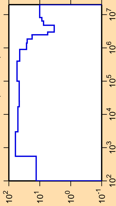
\Delta\sigma/\sigma vs. E for ^{178}\text{Os}(n,\text{nonel.})
