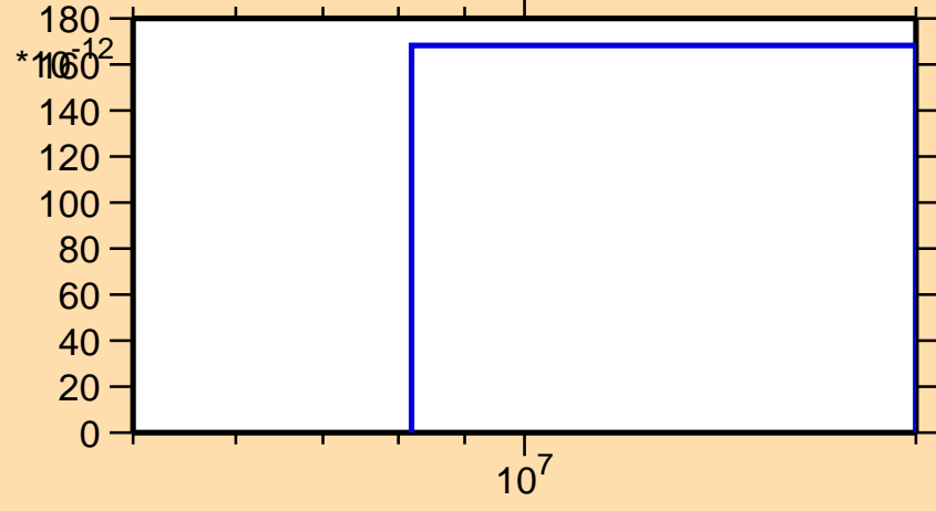
\sigma vs. E for ^{178}\text{Os}(n,\text{pd})
