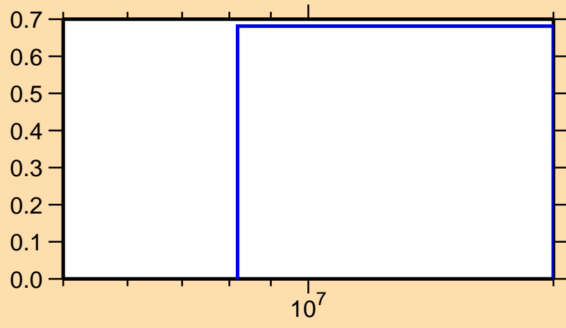
\sigma vs. E for ^{178}\text{Os}(n,2n)
