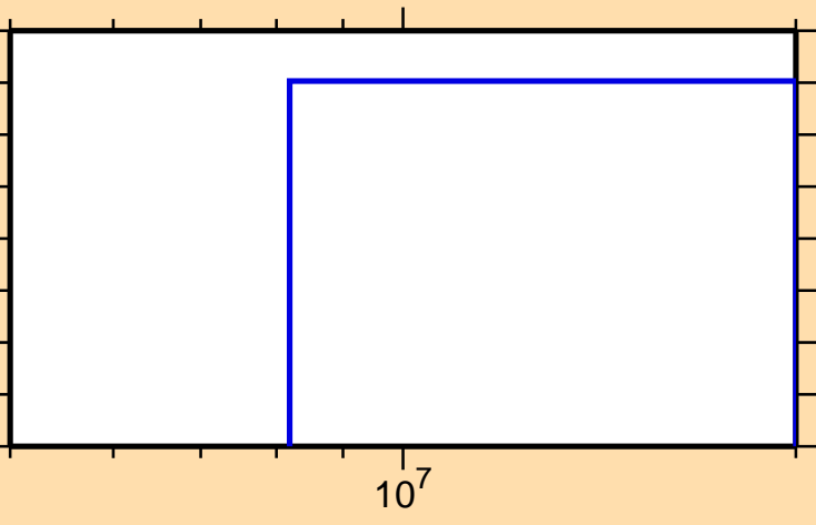
\sigma vs. E for ^{178}\text{Os}(n,t)
