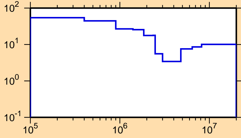
\Delta\sigma/\sigma vs. E for ^{178}\text{Os}(n,\text{nonel.})
