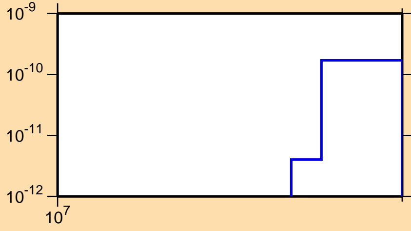
\sigma vs. E for ^{179}\text{Os} (mt 34)
