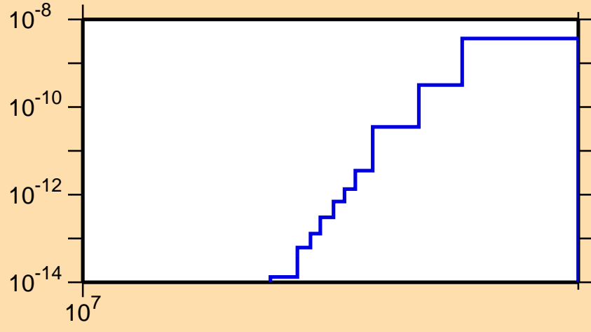
\sigma vs. E for ^{179}\text{Os}(n,\text{pd})
