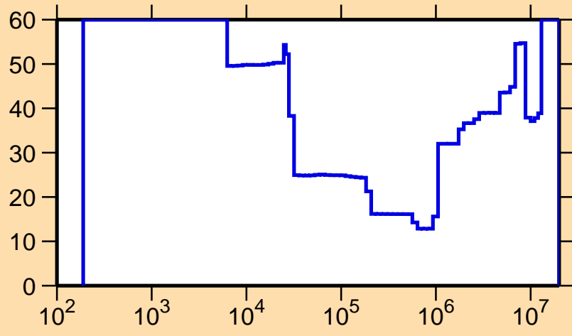
\Delta\sigma/\sigma vs. E for ^{179}\text{Os}(n,\gamma)
