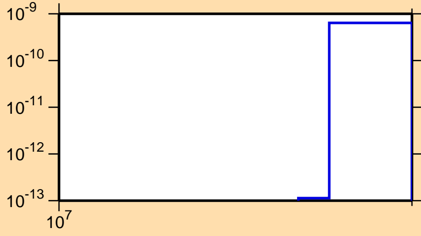
\sigma vs. E for ^{179}\text{Os}(n,nt)
