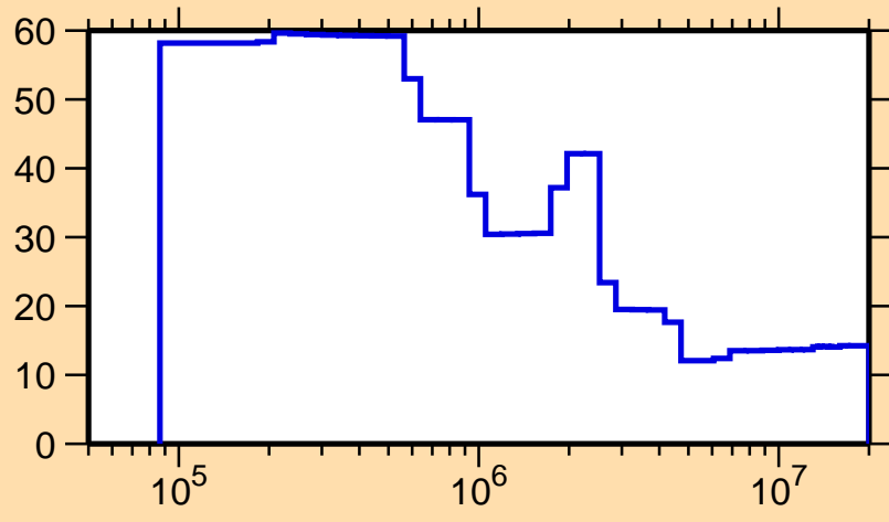
\Delta\sigma/\sigma vs. E for ^{179}\text{Os}(n,n_1)
