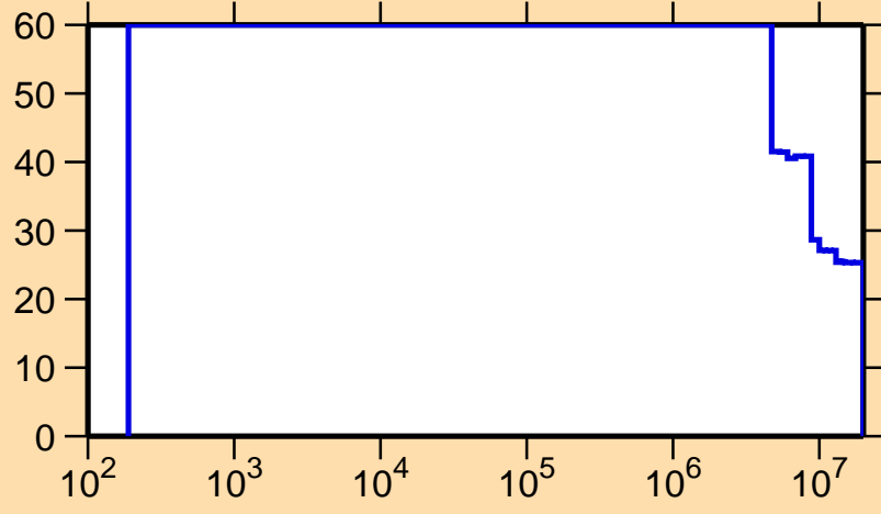
\Delta\sigma/\sigma vs. E for ^{179}\text{Os}(n,p)
