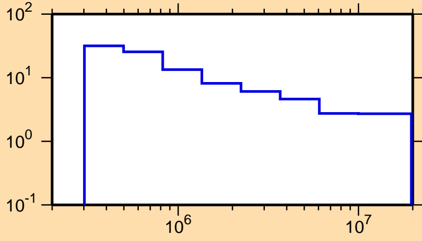
\Delta\sigma/\sigma vs. E for ^{179}\text{Os}(n,n\text{onel.})
