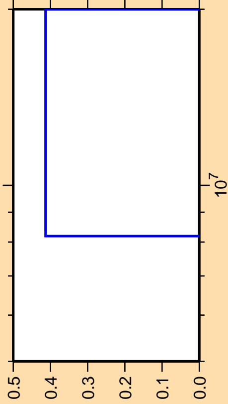
\Delta\sigma/\sigma vs. E for ^{179}\text{Os}(n,3n\alpha)
