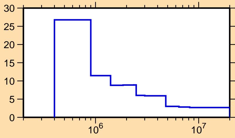
\Delta\sigma/\sigma vs. E for ^{179}\text{Os}(n,\text{nonel.})
