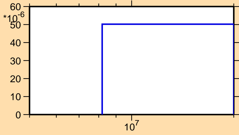
\sigma vs. E for ^{179}\text{Os}(n,3n)
