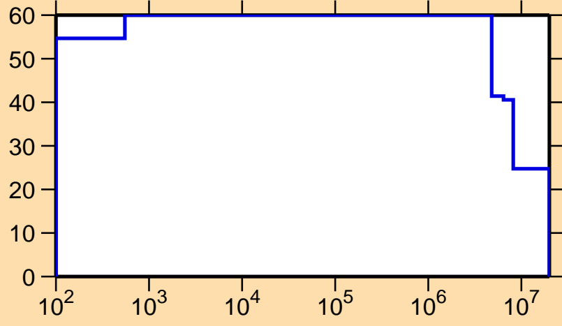
\Delta\sigma/\sigma vs. E for ^{179}\text{Os}(n,p)
