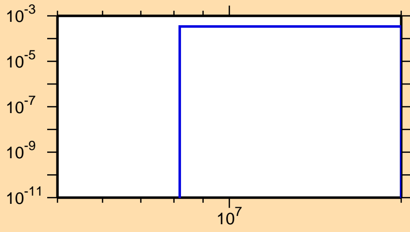
\sigma vs. E for ^{179}\text{Os}(n,2n\alpha)
