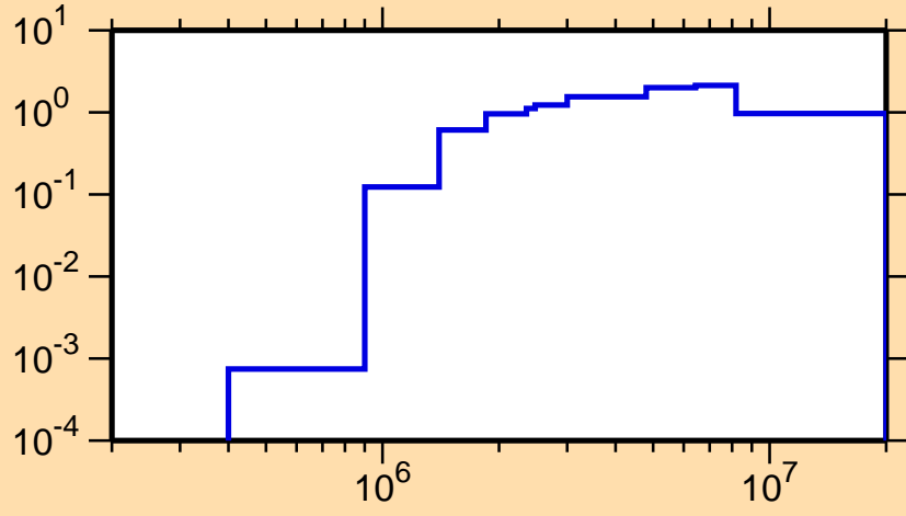
\sigma vs. E for ^{179}\text{Os}(n,n\text{cont.})
