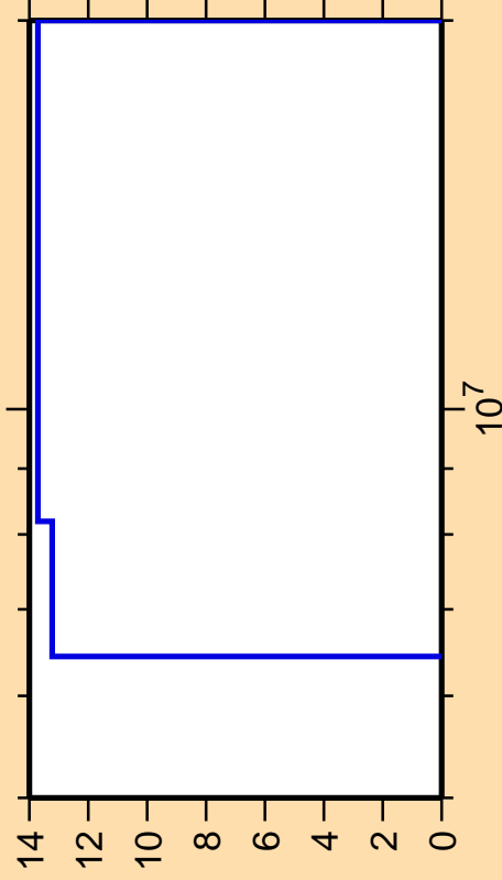
\Delta\sigma/\sigma vs. E for ^{179}\text{Os}(n,n_1)
