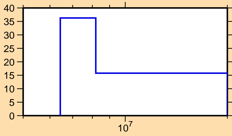
\Delta\sigma/\sigma vs. E for ^{179}\text{Os}(n,2n)
