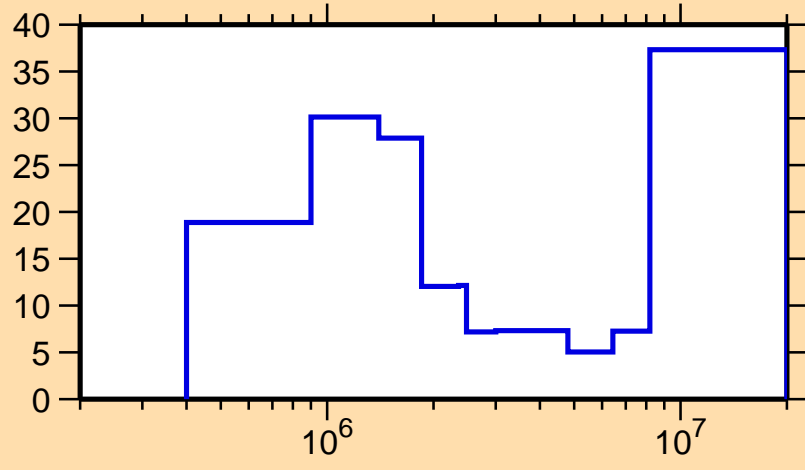
\Delta\sigma/\sigma vs. E for ^{179}\text{Os}(n,n\text{cont.})
