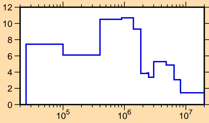
\Delta\sigma/\sigma vs. E for ^{179}\text{Os}(n,\text{tot.})
