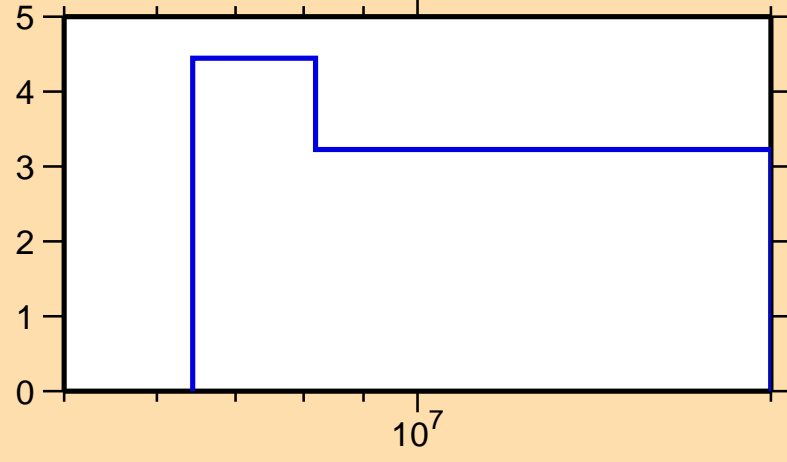
\Delta\sigma/\sigma vs. E for ^{179}\text{Os}(n,\text{el.})
