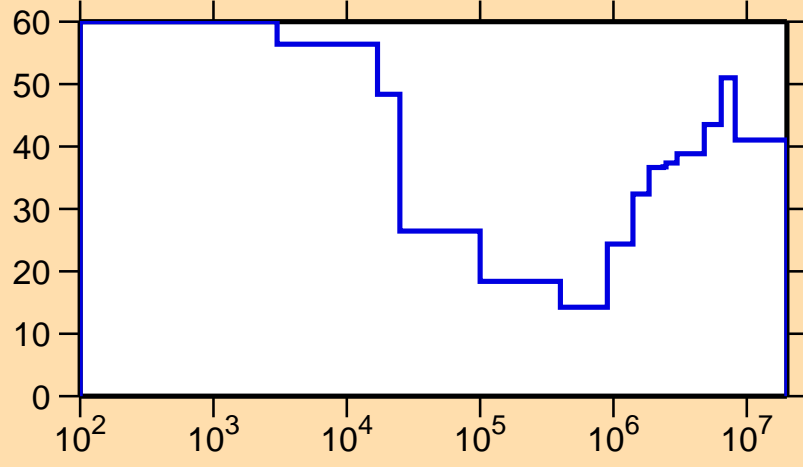
\Delta\sigma/\sigma vs. E for ^{179}\text{Os}(n,\gamma)
