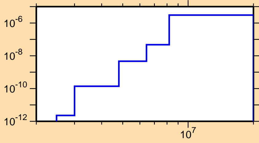
\sigma vs. E for ^{179}\text{Os}(n,p\alpha)
