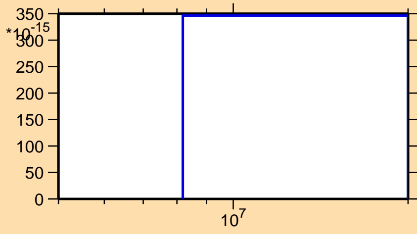
\sigma vs. E for ^{179}\text{Os}(n,3n\alpha)
