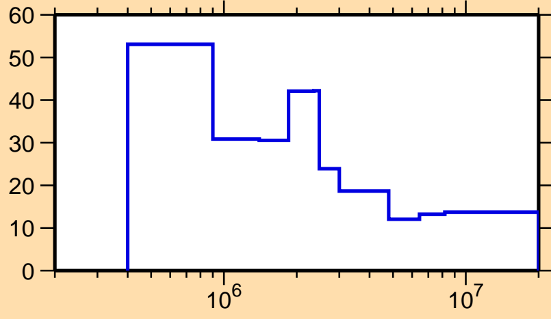
\Delta\sigma/\sigma vs. E for ^{179}\text{Os}(n,n_1)
