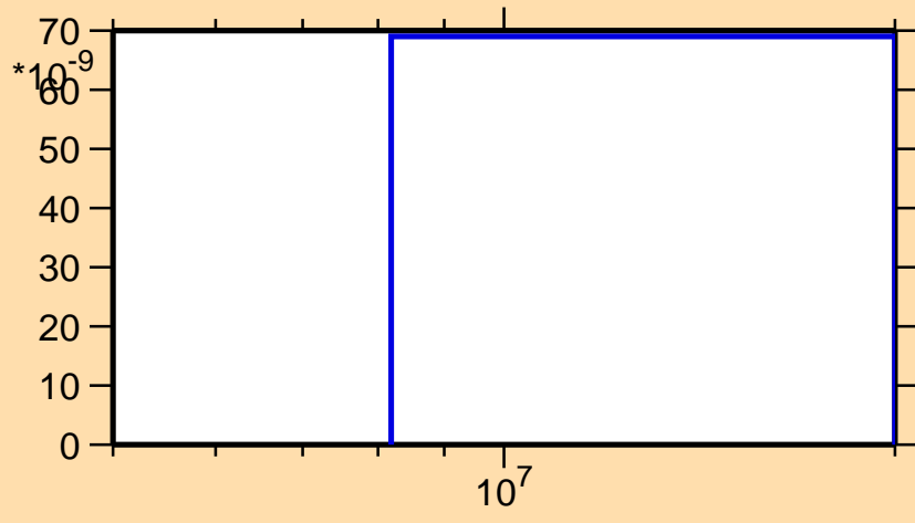
\sigma vs. E for ^{179}\text{Os}(n,\text{He}3)
