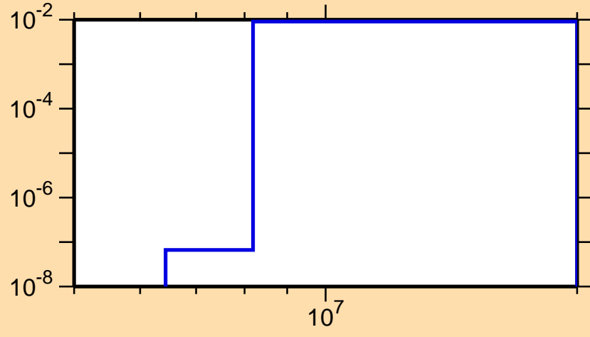
\sigma vs. E for ^{179}\text{Os}(n,np)
