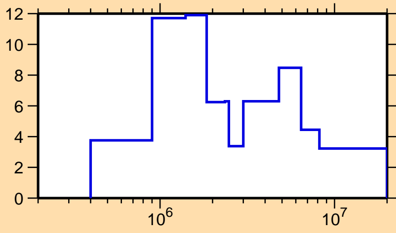
\Delta\sigma/\sigma vs. E for ^{179}\text{Os}(n,\text{el.})
