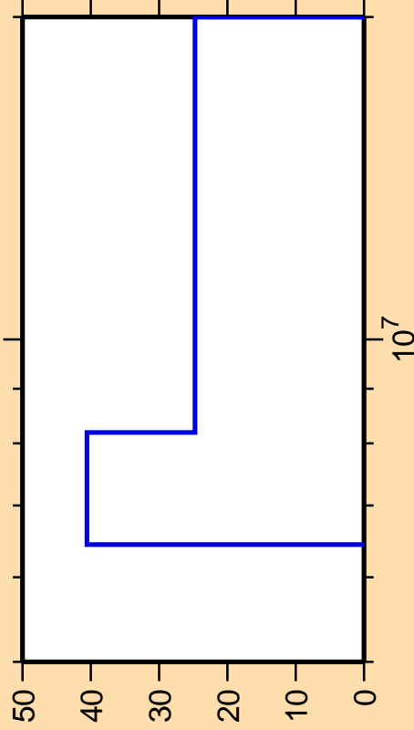
\Delta\sigma/\sigma vs. E for ^{179}\text{Os}(n,p)
