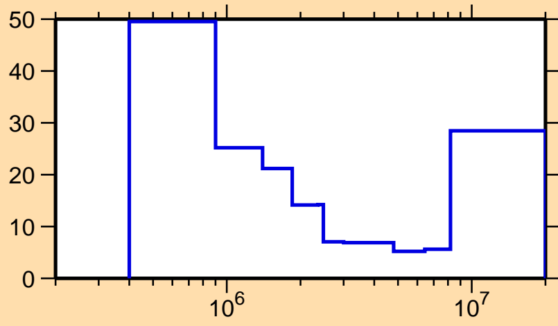
\Delta\sigma/\sigma vs. E for ^{179}\text{Os}(n,\text{inel.})
