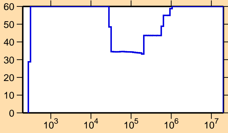
\Delta\sigma/\sigma vs. E for ^{181}\text{Os}(n,\gamma)
