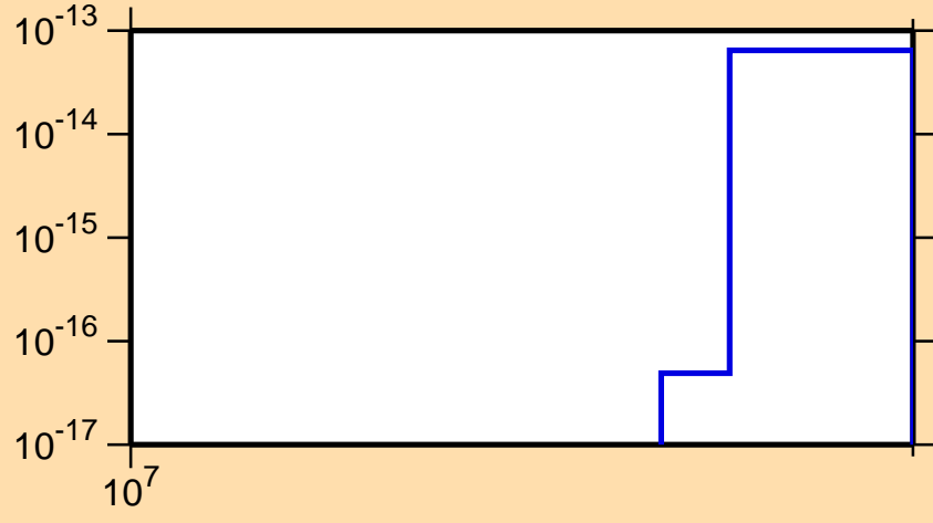
\sigma vs. E for ^{182}\text{Os} (mt 34)
