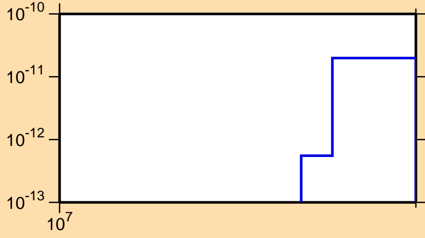
\sigma vs. E for ^{182}\text{Os}(n,\text{pd})
