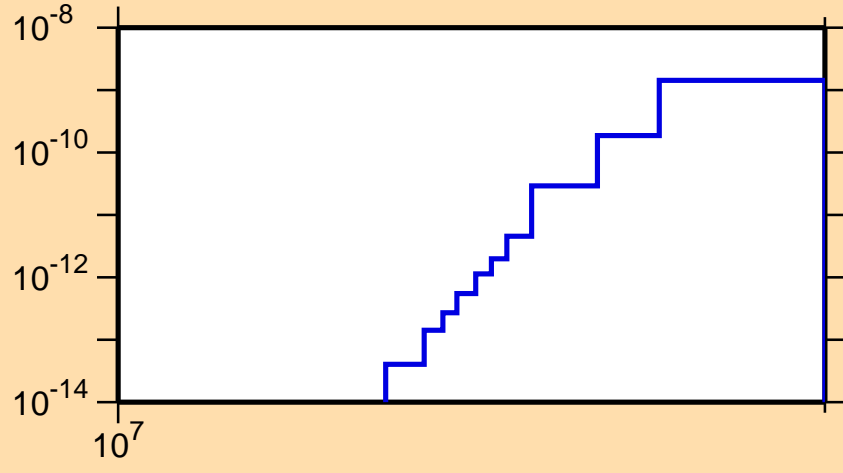
\sigma vs. E for ^{182}\text{Os} (mt 45)
