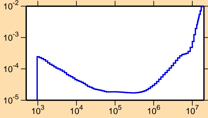
\sigma vs. E for ^{182}\text{Os}(n,\alpha)
