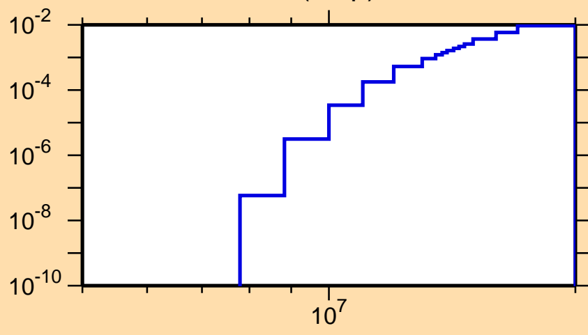
\sigma vs. E for ^{182}\text{Os}(n,np)
