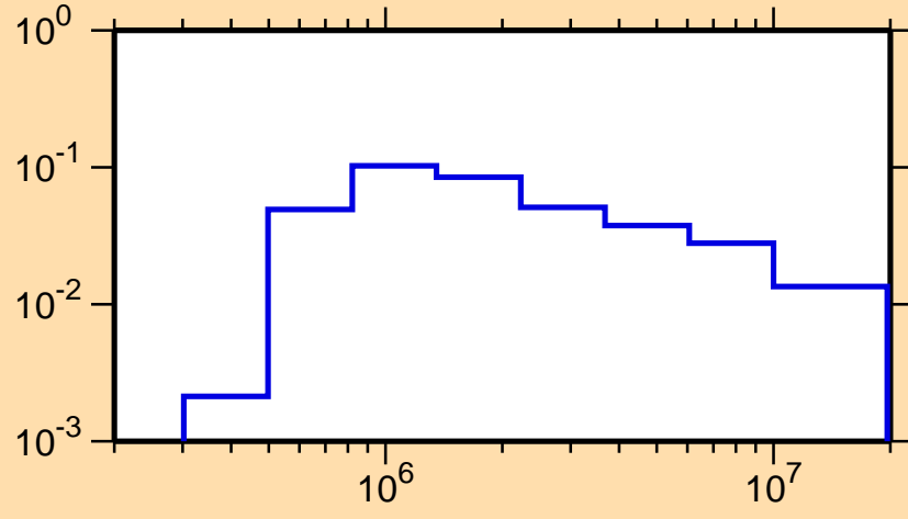
\sigma vs. E for ^{182}\text{Os}(n,n_2)
