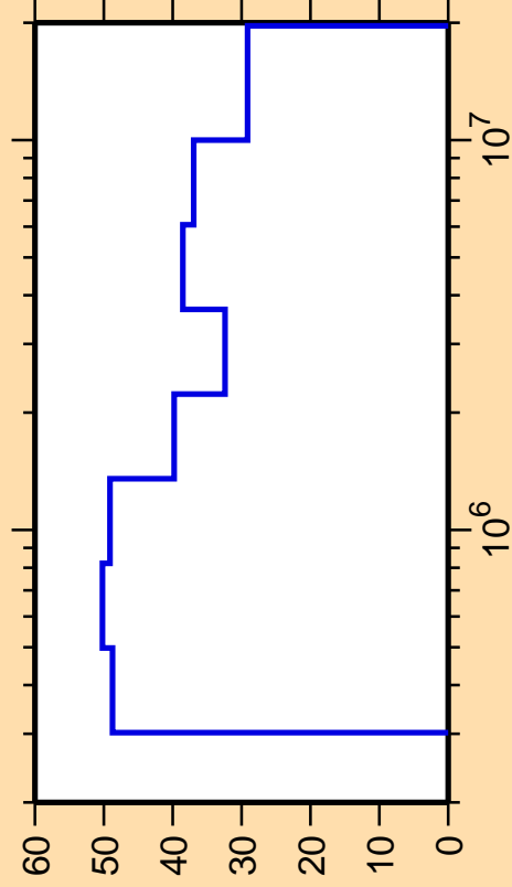
\Delta\sigma/\sigma vs. E for ^{182}\text{Os}(n,n_2)
