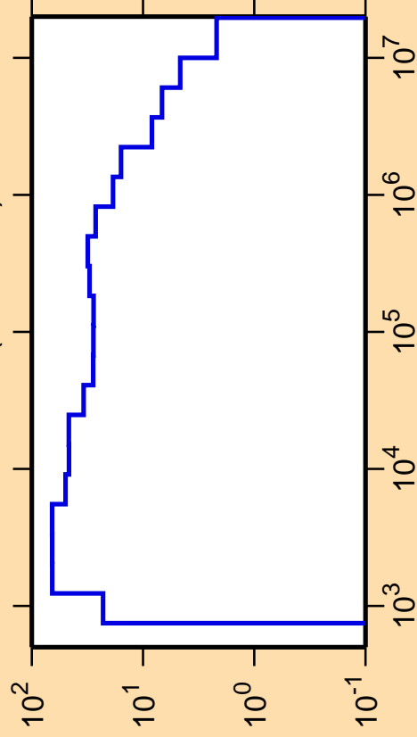
\Delta\sigma/\sigma vs. E for ^{182}\text{Os}(n,\text{nonel.})
