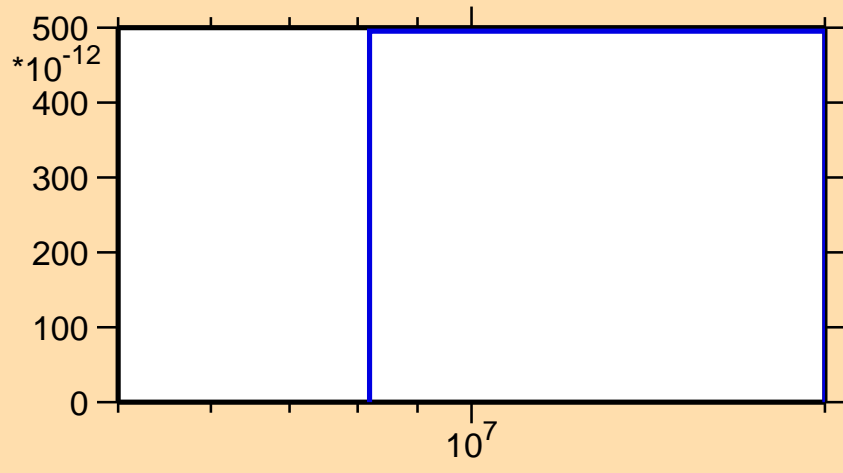
\sigma vs. E for ^{182}\text{Os}(n,\text{nd})
