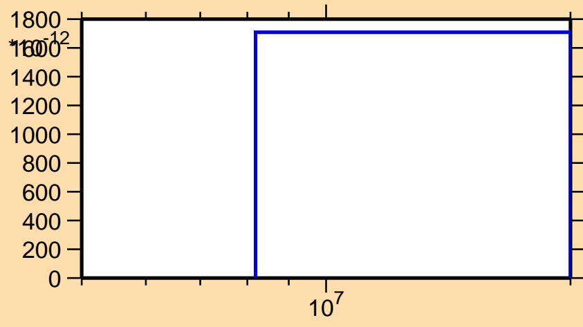
\sigma vs. E for ^{182}\text{Os}(n,2np)
