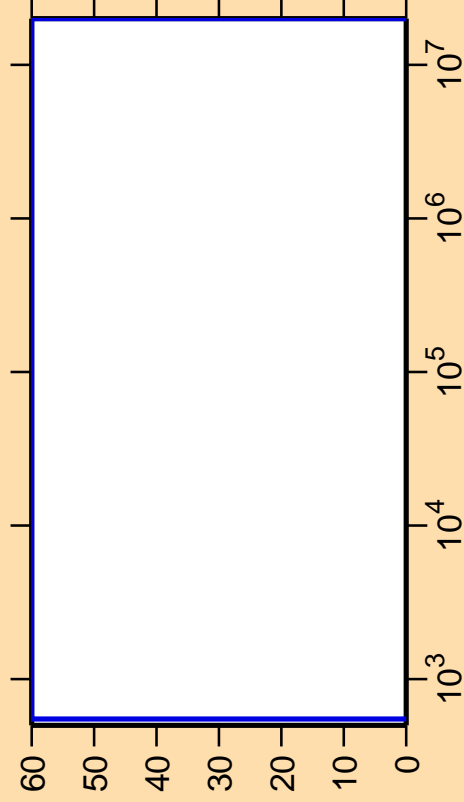
\Delta\sigma/\sigma vs. E for ^{182}\text{Os}(n,\alpha)
