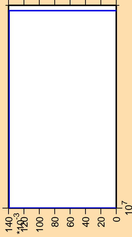
\Delta\sigma/\sigma vs. E for ^{183}\text{Os}(n,3n\alpha)
