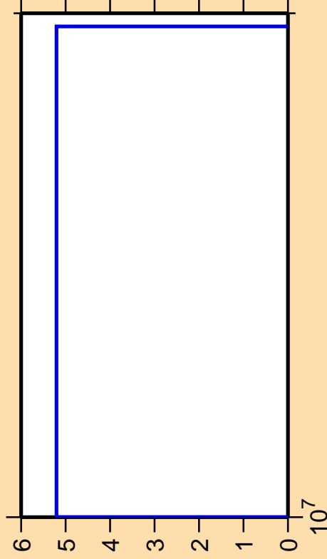
\Delta\sigma/\sigma vs. E for ^{183}\text{Os}(\text{mt117})
