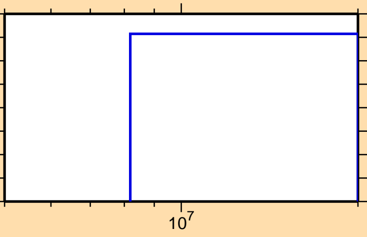
\sigma vs. E for ^{183}\text{Os}(n,pd)
