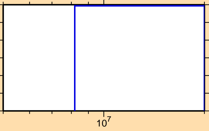
\sigma vs. E for ^{183}\text{Os}(n,t)
