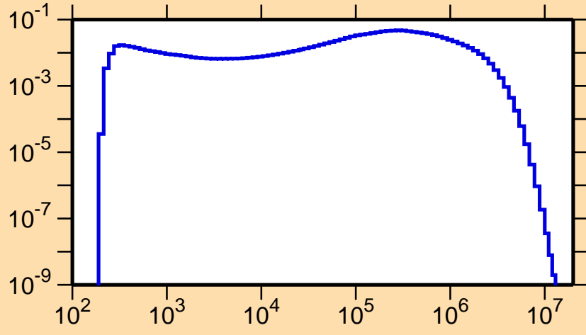
\sigma vs. E for ^{183}\text{Os}(n,n_1)
