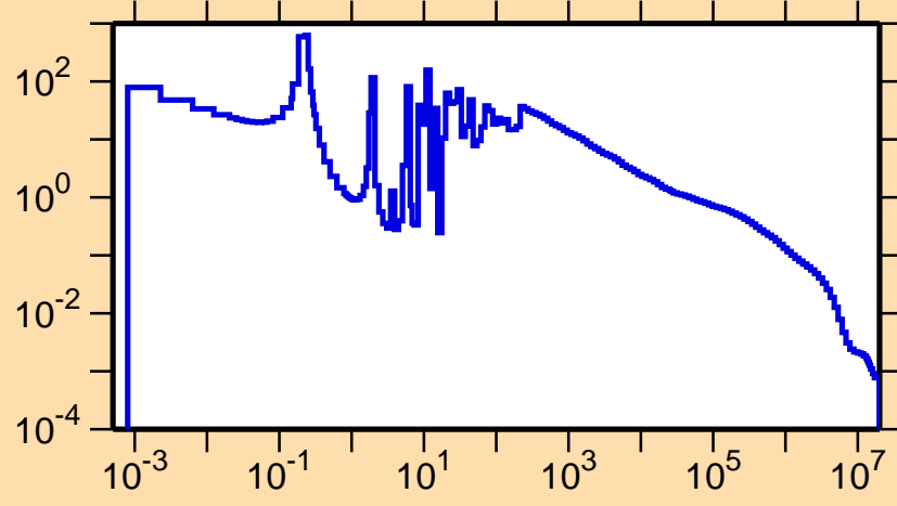
\sigma vs. E for ^{183}\text{Os}(n,\gamma)
