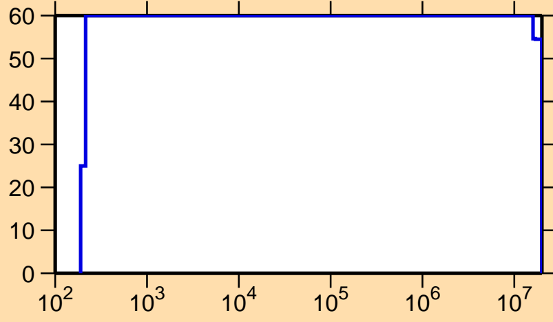
\Delta\sigma/\sigma vs. E for ^{183}\text{Os}(n,p)
