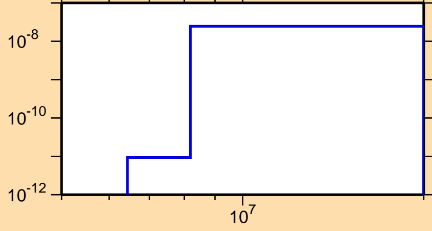
\sigma vs. E for ^{183}\text{Os}(n,p\alpha)
