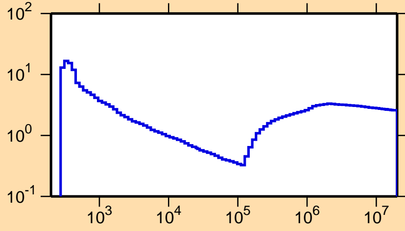
\sigma vs. E for ^{184}\text{Os}(n,\text{nonel.})
