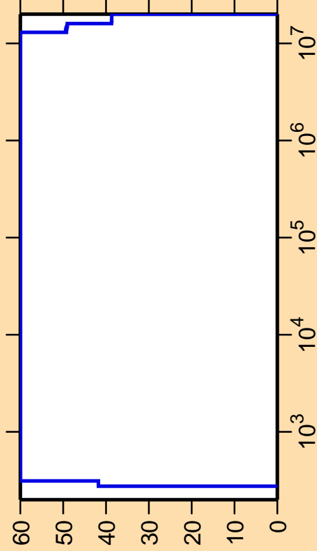
\Delta\sigma/\sigma vs. E for ^{184}\text{Os}(n,\alpha)
