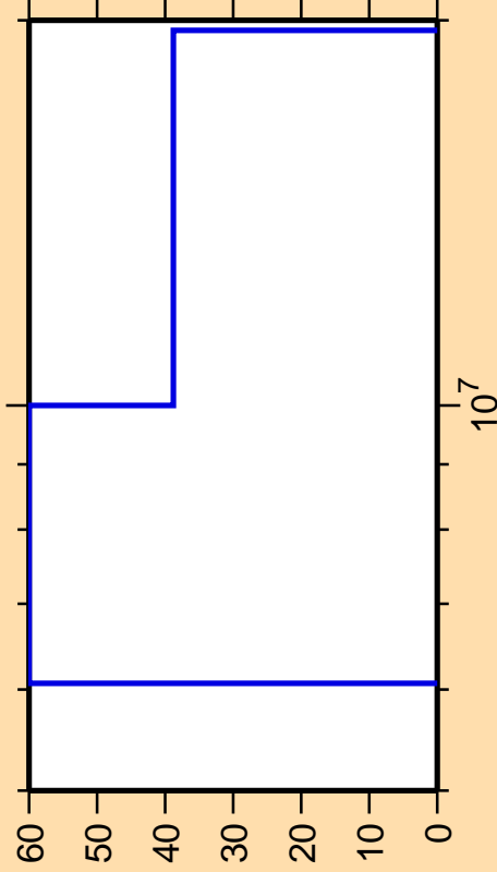
\Delta\sigma/\sigma vs. E for ^{184}\text{Os}(n,np)
