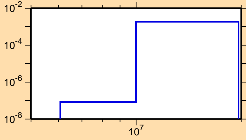
\sigma vs. E for ^{184}\text{Os}(n,np)
