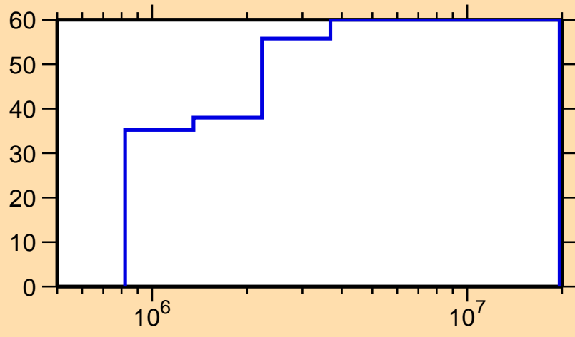
\Delta\sigma/\sigma vs. E for ^{184}\text{Os}(n,\gamma)
