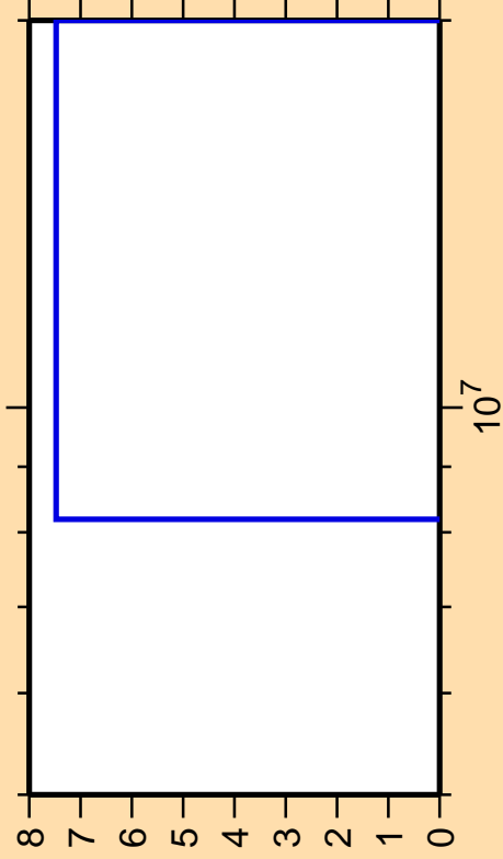
\Delta\sigma/\sigma vs. E for ^{184}\text{Os}(n,2n)
