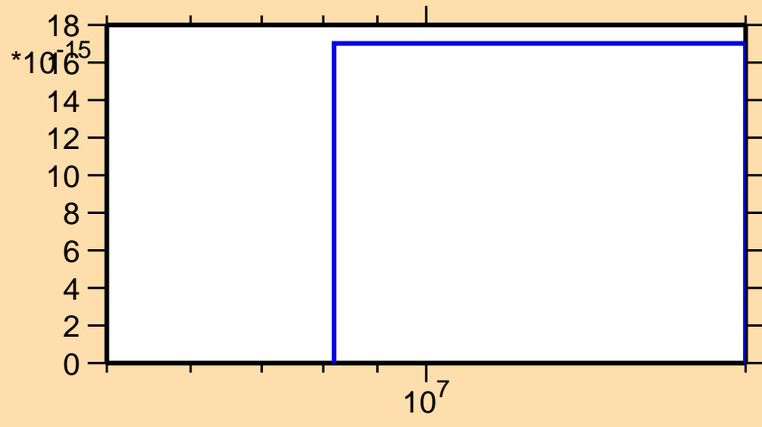
\sigma vs. E for ^{184}\text{Os}(n,pd)
