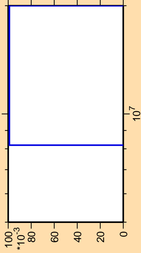
\Delta\sigma/\sigma vs. E for ^{184}\text{Os}(n,pd)
