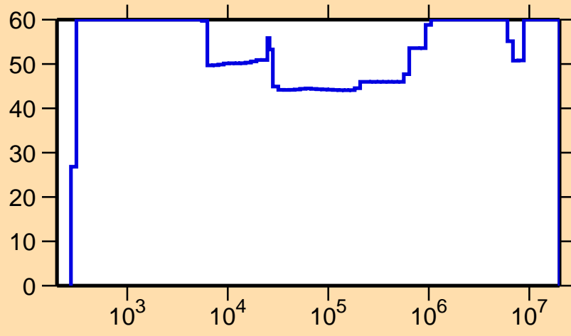
\Delta\sigma/\sigma vs. E for ^{185}\text{Os}(n,\gamma)
