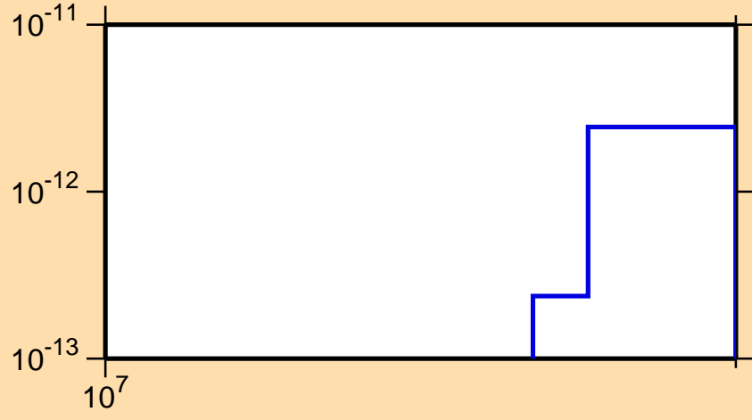
\sigma vs. E for ^{185}\text{Os}(\text{mt117})
