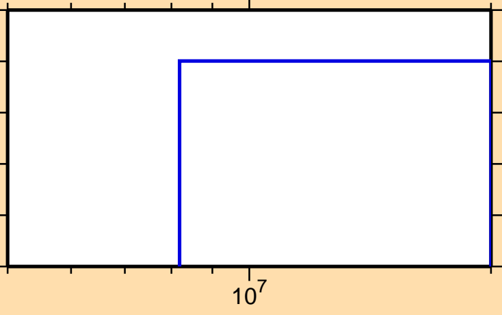
\sigma vs. E for ^{185}\text{Os}(n,p\alpha)
