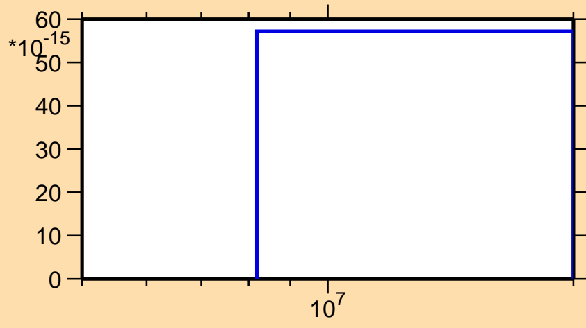
\sigma vs. E for ^{185}\text{Os}(n,3n\alpha)
