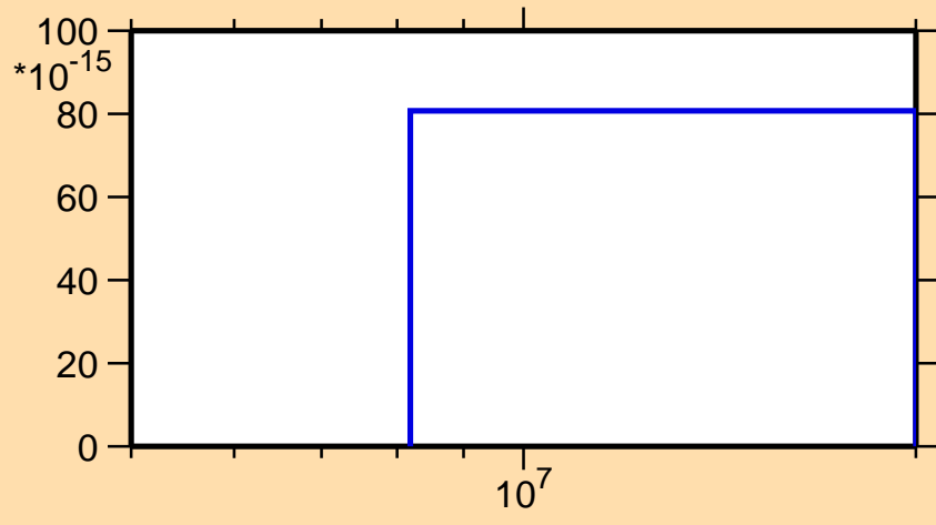
\sigma vs. E for ^{186}\text{Os}(\text{mt117})
