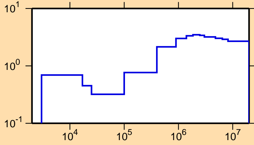
\sigma vs. E for ^{186}\text{Os}(n,\text{nonel.})
