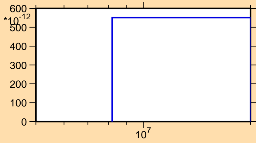
\sigma vs. E for ^{186}\text{Os}(n,2np)
