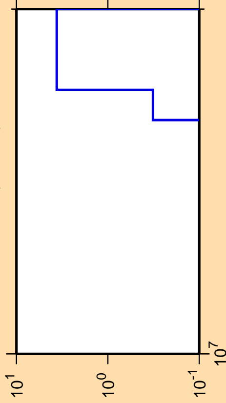
\Delta\sigma/\sigma vs. E for ^{187}\text{Os}(\text{mt117})
