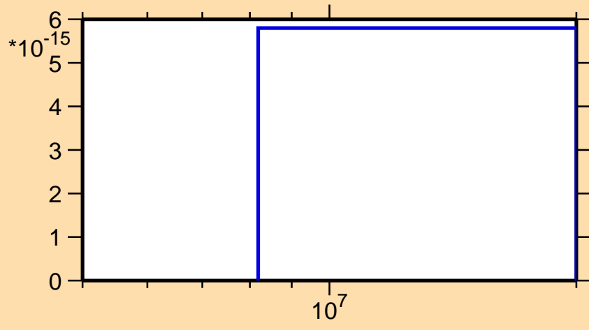
\sigma vs. E for ^{187}\text{Os}(\text{mt117})
