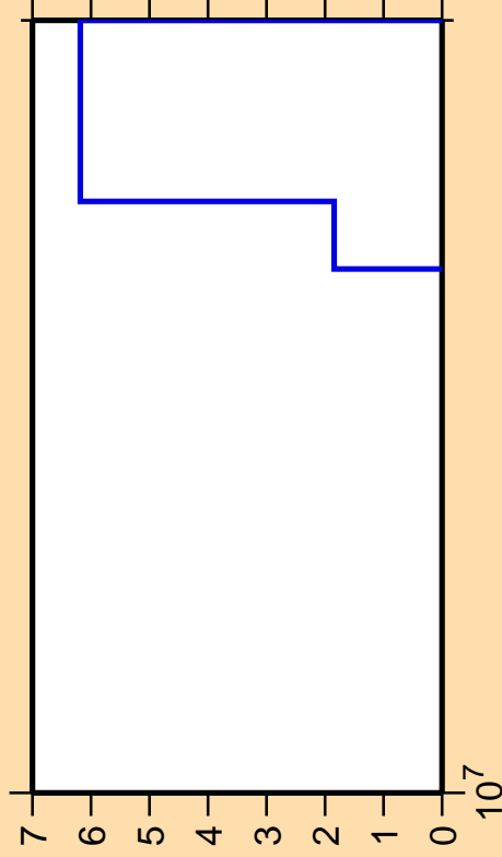
\Delta\sigma/\sigma vs. E for ^{188}\text{Os}(n,p\alpha)
