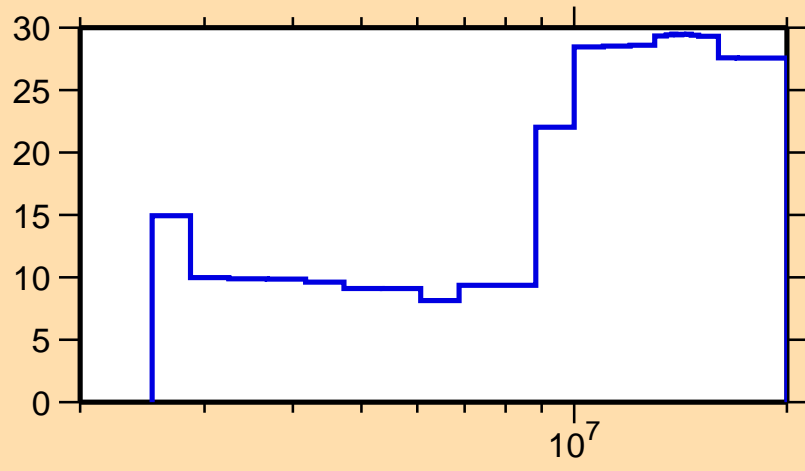
\Delta\sigma/\sigma vs. E for ^{188}\text{Os}(n,n\text{cont.})
