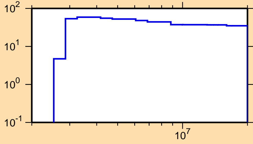
\Delta\sigma/\sigma vs. E for ^{189}\text{Os}(n,p)
