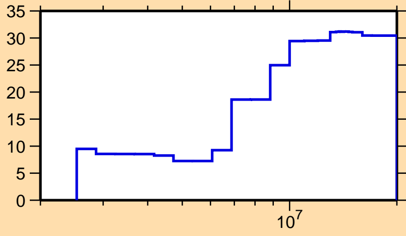
\Delta\sigma/\sigma vs. E for ^{189}\text{Os}(n,n\text{cont.})
