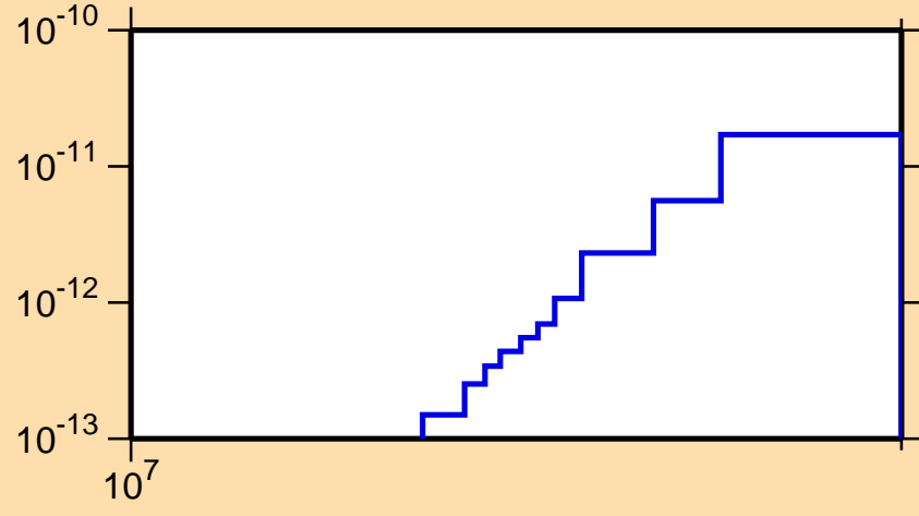
\sigma vs. E for ^{189}\text{Os}(n,p\alpha)
