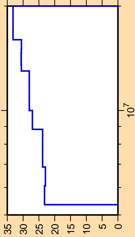
\Delta\sigma/\sigma vs. E for ^{189}\text{Os}(n,n_1)
