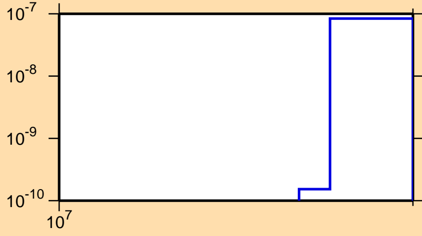
\sigma vs. E for ^{189}\text{Os}(n,nt)
