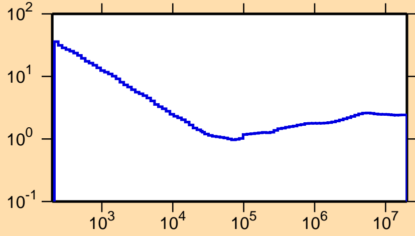
\sigma vs. E for ^{189}\text{Os}(n,\text{nonel.})
