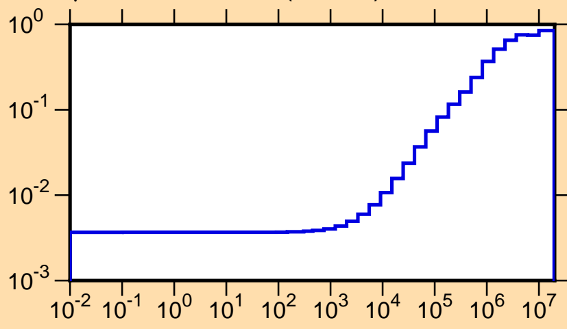
\mu vs. E for ^{189}\text{Os}(\text{mt251})
