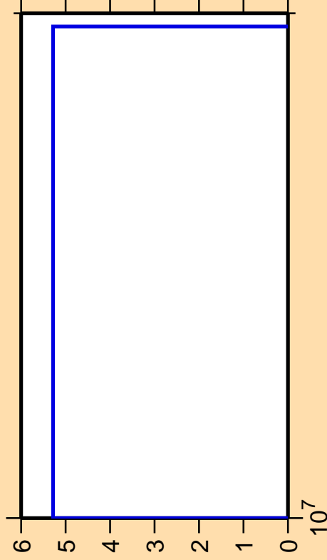
\Delta\sigma/\sigma vs. E for ^{189}\text{Os}(n,p\alpha)
