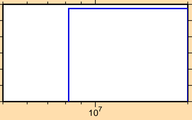
\sigma vs. E for ^{189}\text{Os}(n,\text{He}3)
