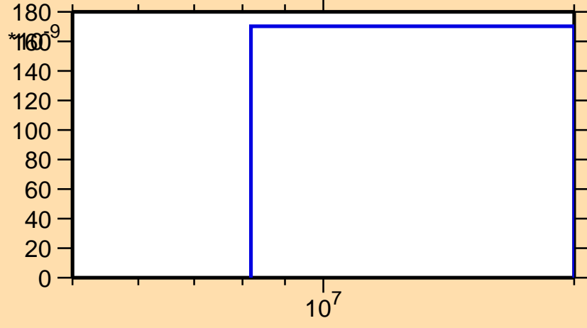
\sigma vs. E for ^{189}\text{Os}(n,2n\alpha)
