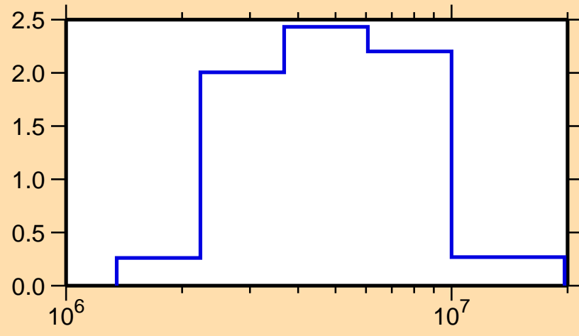
\sigma vs. E for ^{190}\text{Os}(n,n\text{cont.})
