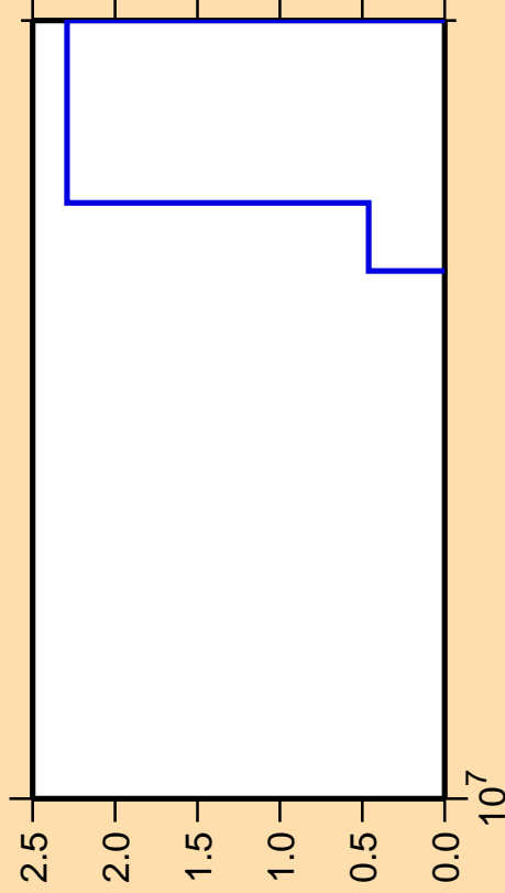
\Delta\sigma/\sigma vs. E for ^{190}\text{Os}(n,p\alpha)
