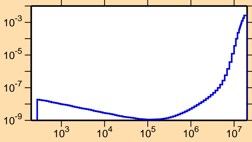
\sigma vs. E for ^{190}\text{Os}(n,\alpha)
