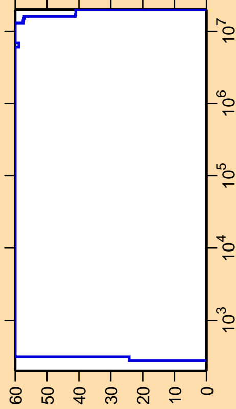
\Delta\sigma/\sigma vs. E for ^{190}\text{Os}(n,\alpha)
