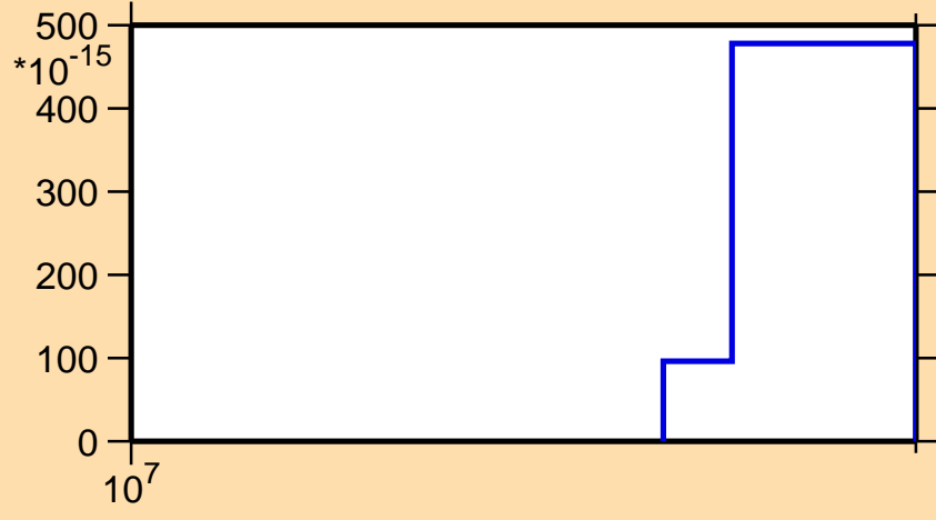
\sigma vs. E for ^{190}\text{Os}(n,p\alpha)
