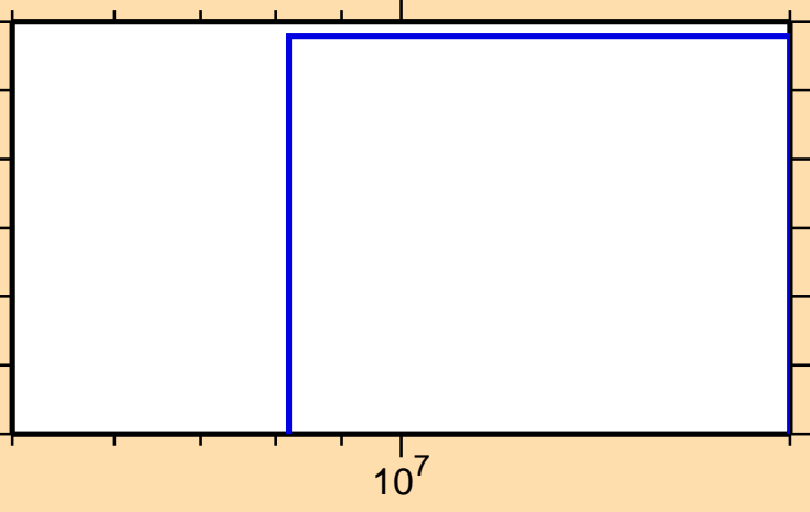
\sigma vs. E for ^{190}\text{Os}(n,t)
