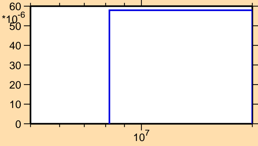
\sigma vs. E for ^{190}\text{Os}(n,t)
