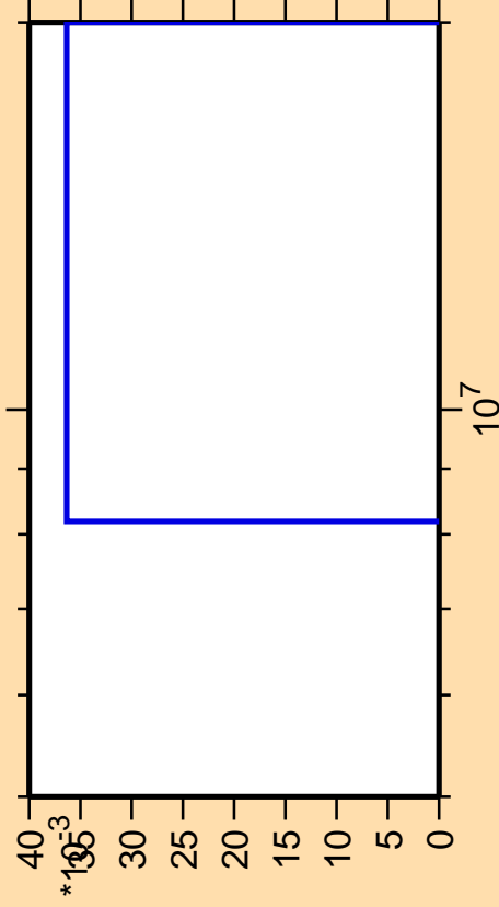
\Delta\sigma/\sigma vs. E for ^{190}\text{Os}(n,p\alpha)
