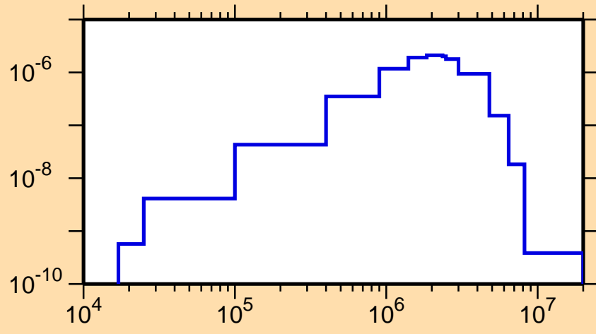
\sigma vs. E for ^{190}\text{Os}(n,n_1)
