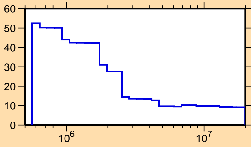
\Delta\sigma/\sigma vs. E for ^{191}\text{Os}(n,n\text{onel.})
