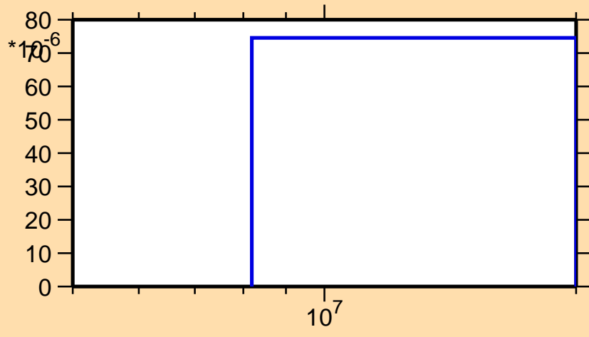
\sigma vs. E for ^{191}\text{Os}(n,d)
