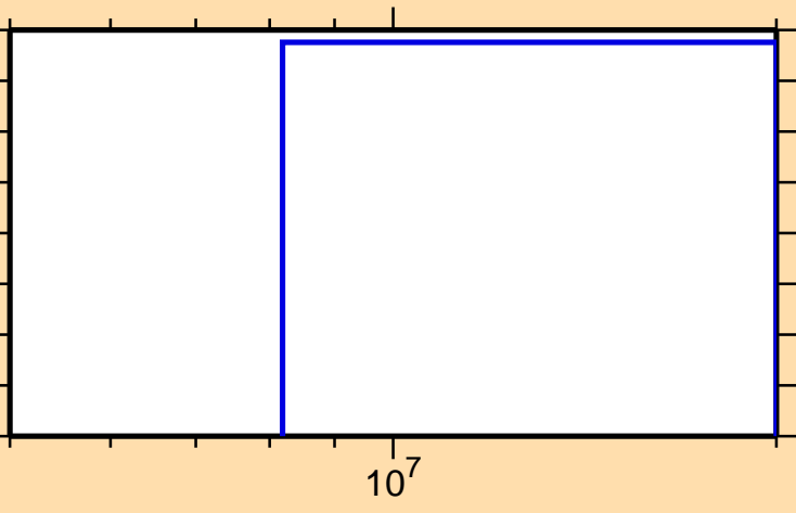
\sigma vs. E for ^{191}\text{Os}(n,\text{He}3)
