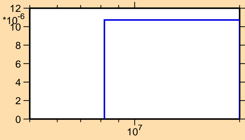
\sigma vs. E for ^{191}\text{Os}(n,t)
