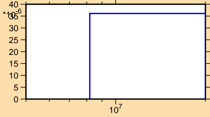
\sigma vs. E for ^{191}\text{Os}(n,np)
