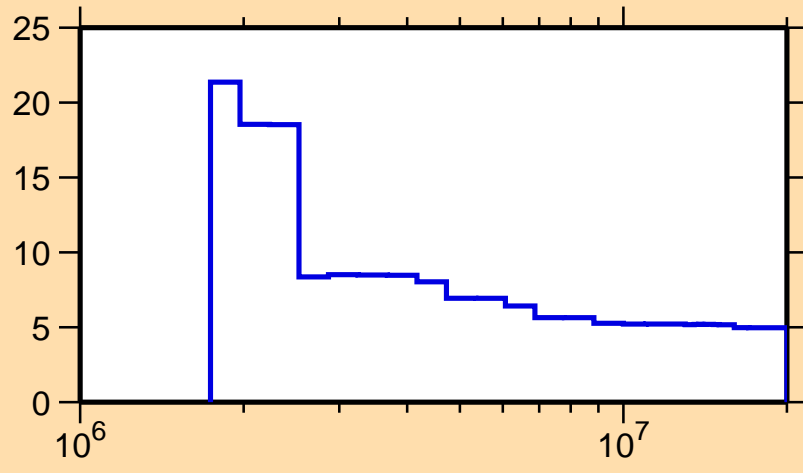
\Delta\sigma/\sigma vs. E for ^{192}\text{Os}(n,n\text{onel.})
