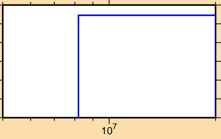
\sigma vs. E for ^{192}\text{Os}(n,2n\alpha)
