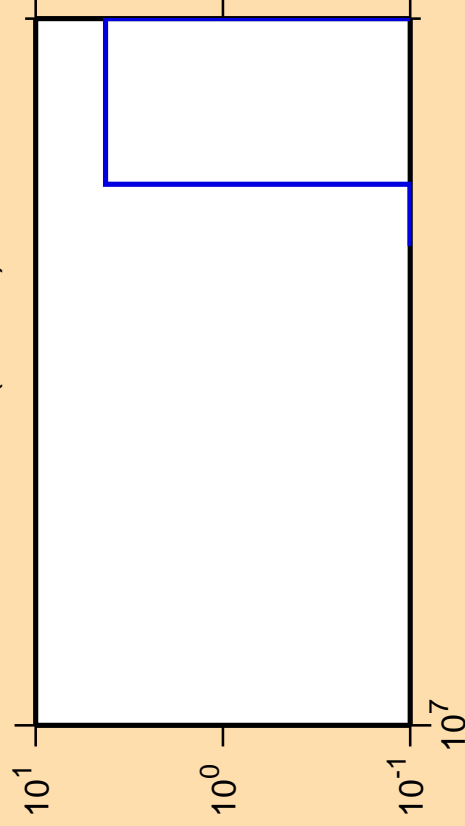
\Delta\sigma/\sigma vs. E for ^{192}\text{Os}(n,3n\alpha)
