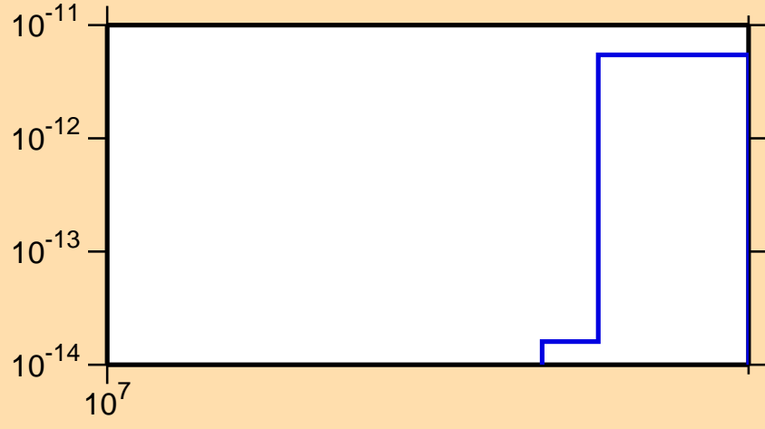
\sigma vs. E for ^{192}\text{Os}(n,3n\alpha)
