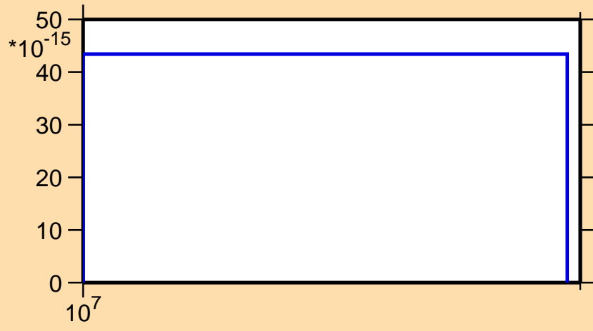
\sigma vs. E for ^{192}\text{Os}(n,3n\alpha)
